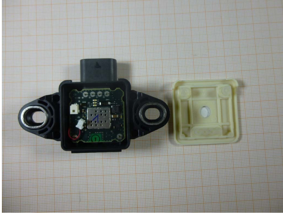
Photo 1: EUT cover removed
