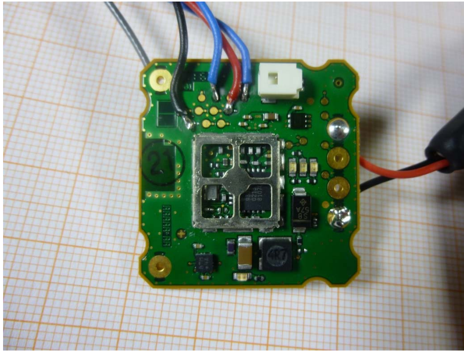
Photo 3: PCB front side view without shielding
