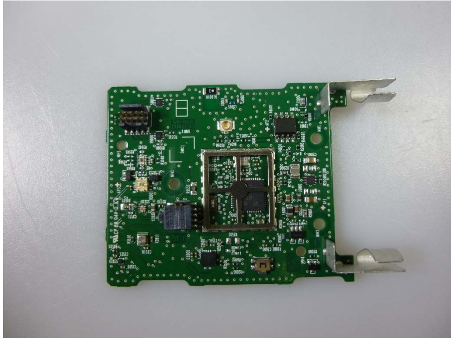
Photo 7: PCB front side view without shielding
