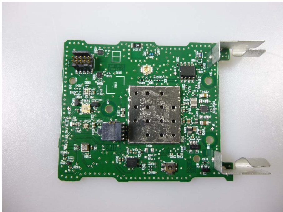
Photo 6: PCB front side view with shielding
