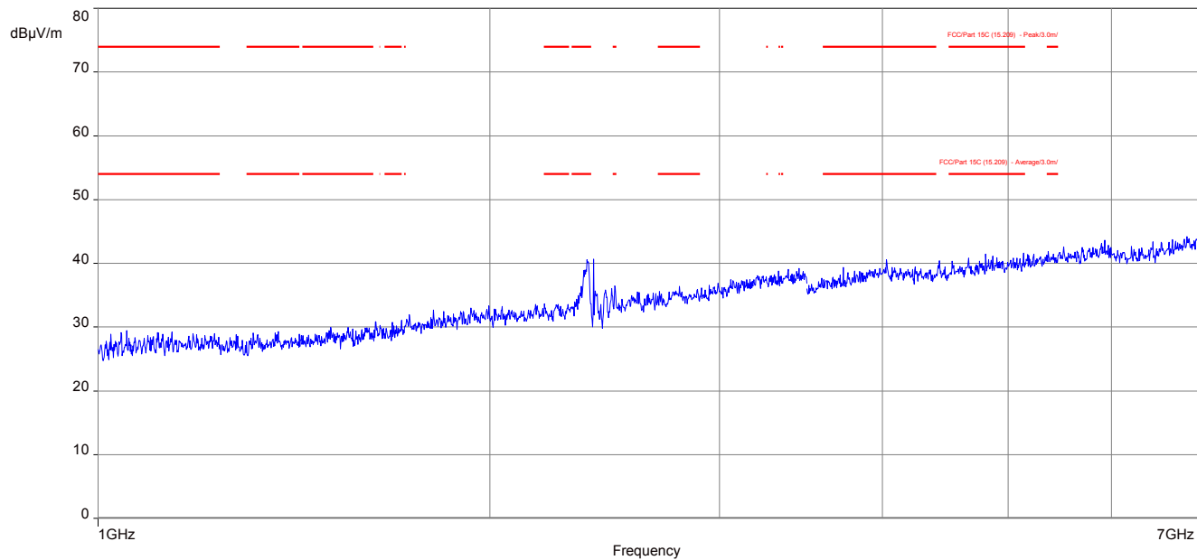
Plot 1: 1 GHz to 7 GHz, TX mode, 2402 MHz, vertical & horizontal polarization
