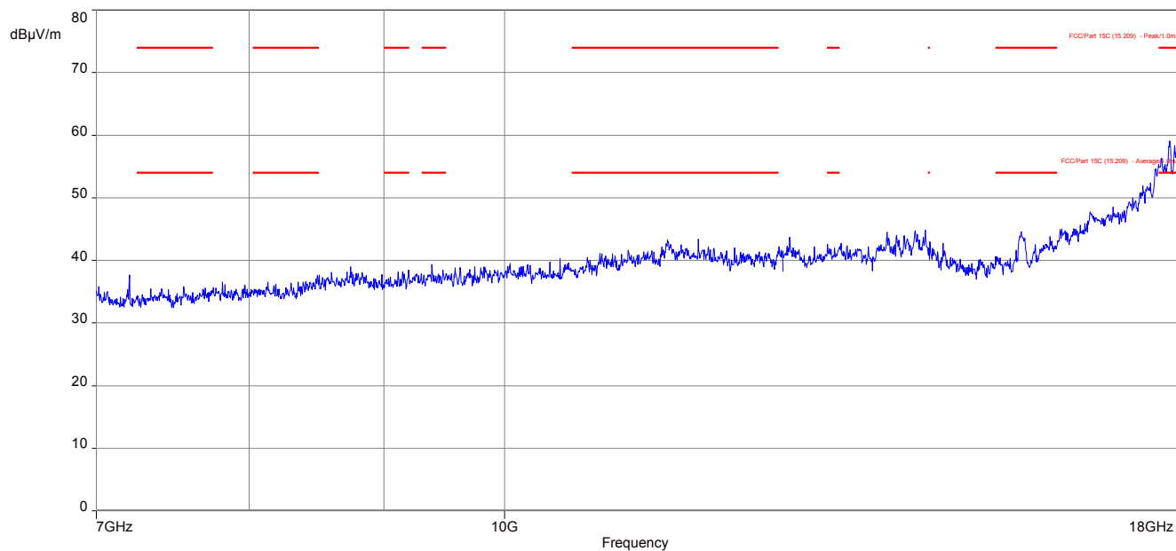
Plot 2: 7 GHz to 18 GHz, TX mode, 2402 MHz, vertical & horizontal polarization
