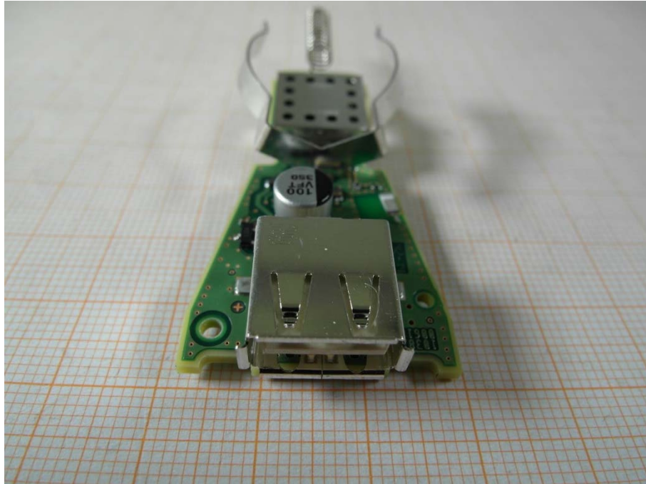
Photo 1: PCB front view
