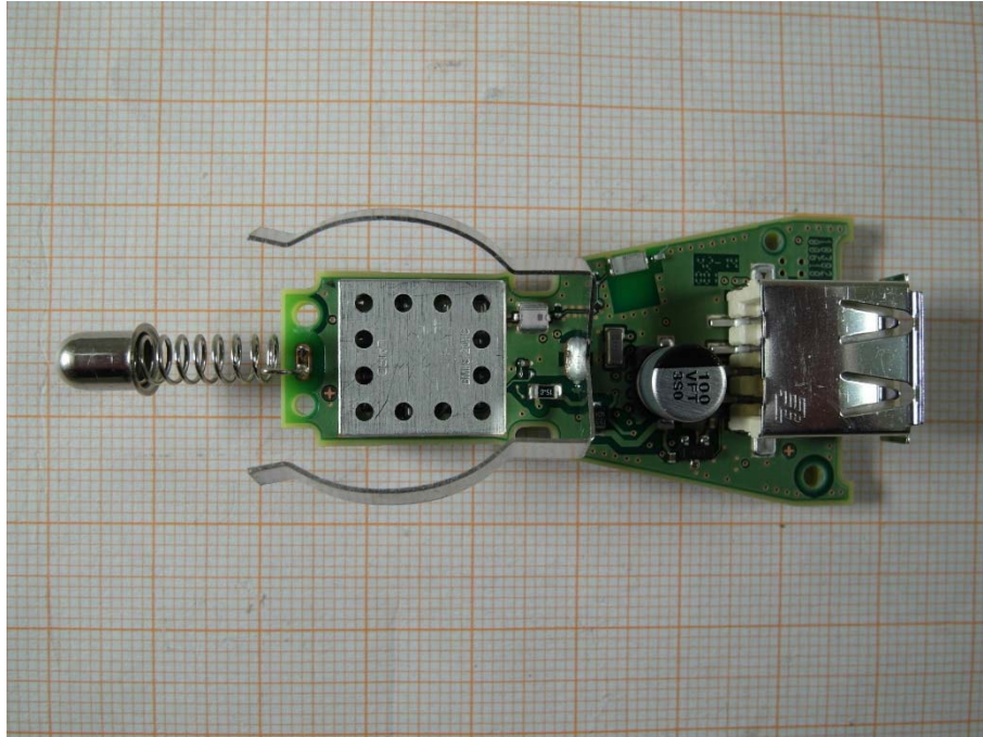
Photo 3: PCB bottom side view (with shielding)
