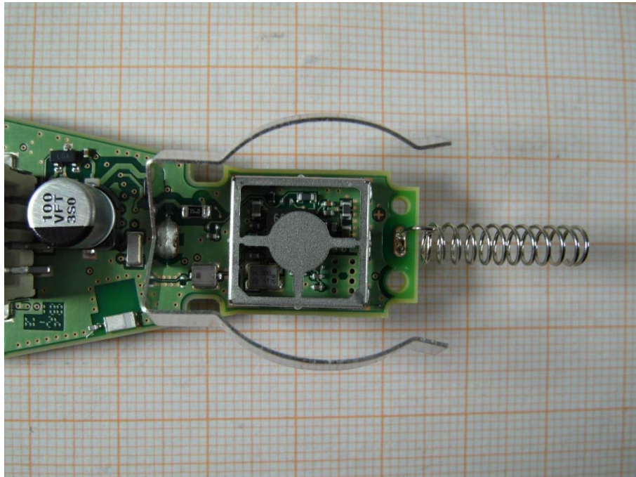
Photo 4: PCB bottom side view (without shielding)
