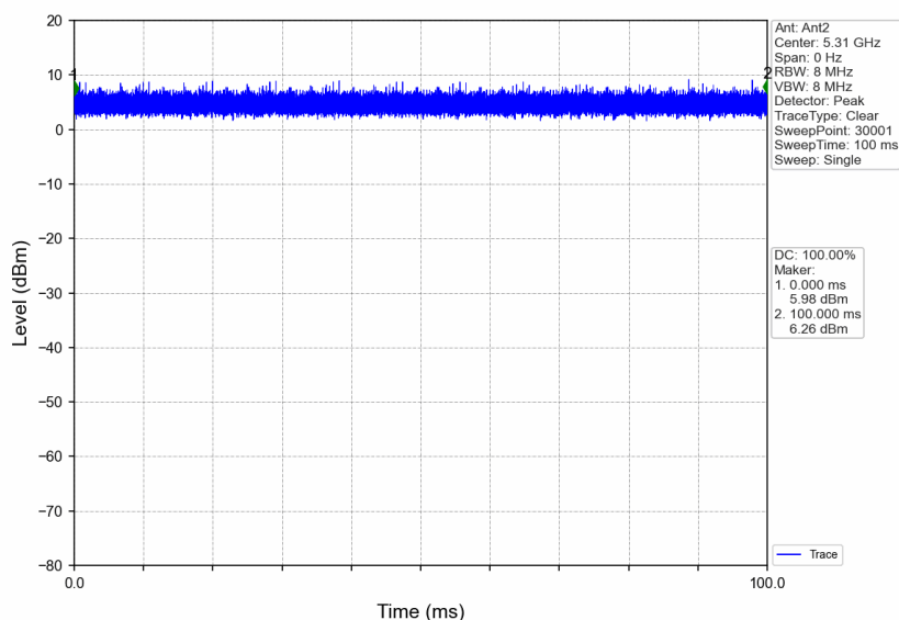
802.11n(HT40)_HCH_5310MHz_Ant2_NTNV
