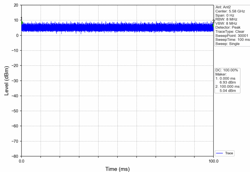
802.11ac(VHT20)_MCH_5580MHz_Ant2_NTNV
