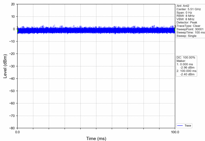
802.11ac(VHT40)_LCH_5510MHz_Ant2_NTNV
