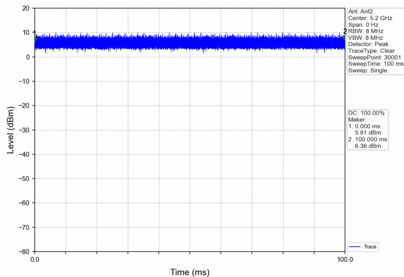
802.11ac(VHT20)_MCH_5200MHz_Ant2_NTNV
