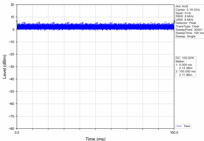
802.11ac(VHT40)_LCH_5190MHz_Ant2_NTNV
