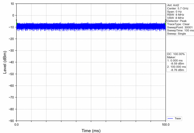
802.11ac(VHT20)_LCH_5745MHz_Ant2_NTNV
