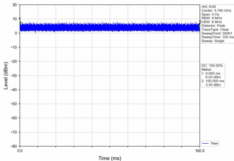
802.11n(HT20)_MCH_5785MHz_Ant2_NTNV
