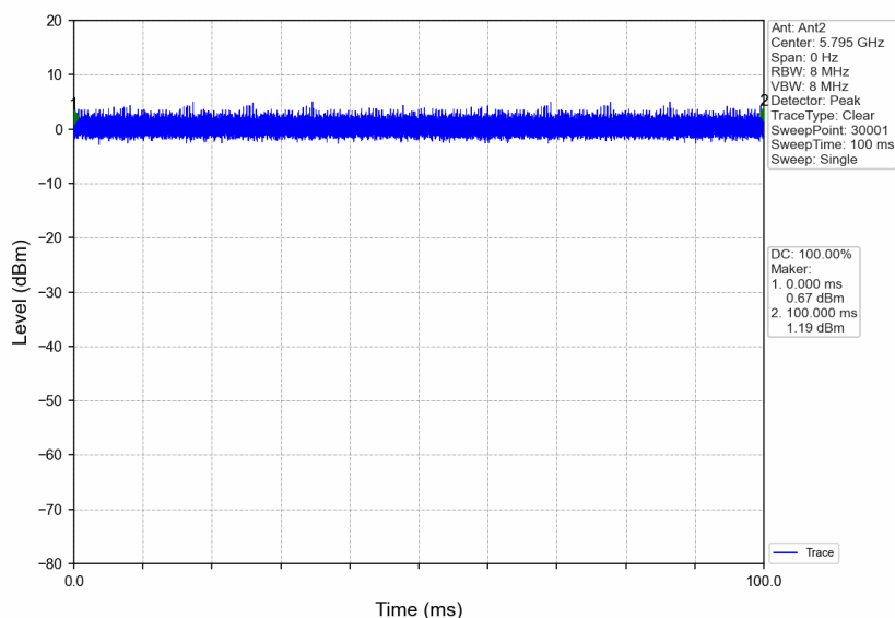
802.11ac(VHT40)_HCH_5795MHz_Ant2_NTNV
