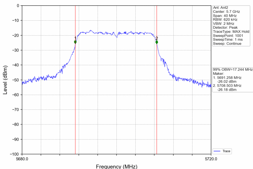
802.11ac(VHT20)_HCH_5700MHz_Ant2_NTNV
