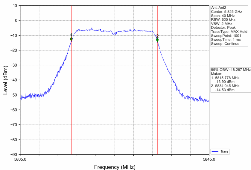
802.11ac(VHT20)_HCH_5825MHz_Ant2_NTNV
