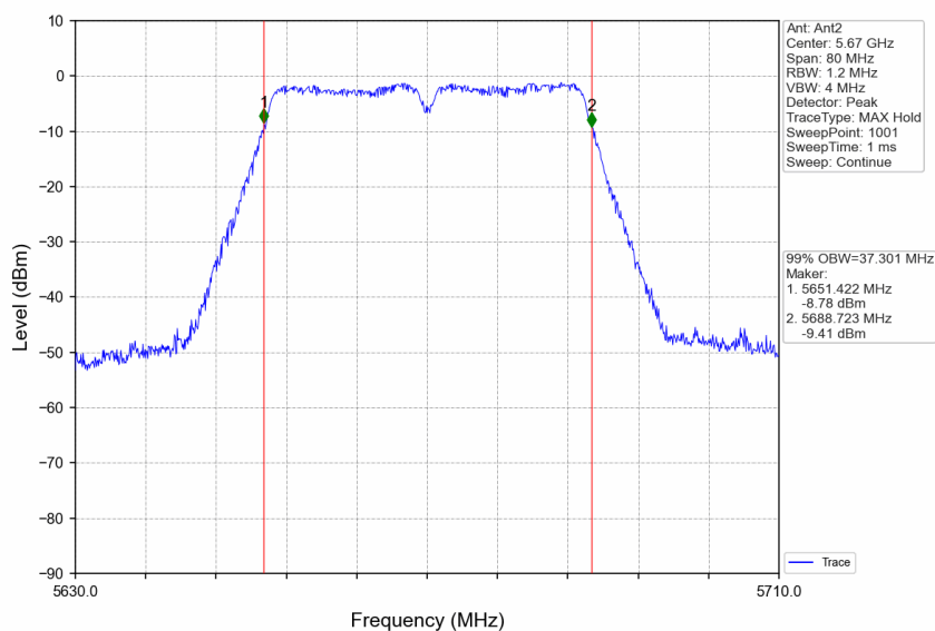
802.11ac(VHT40)_HCH_5670MHz_Ant2_NTNV
