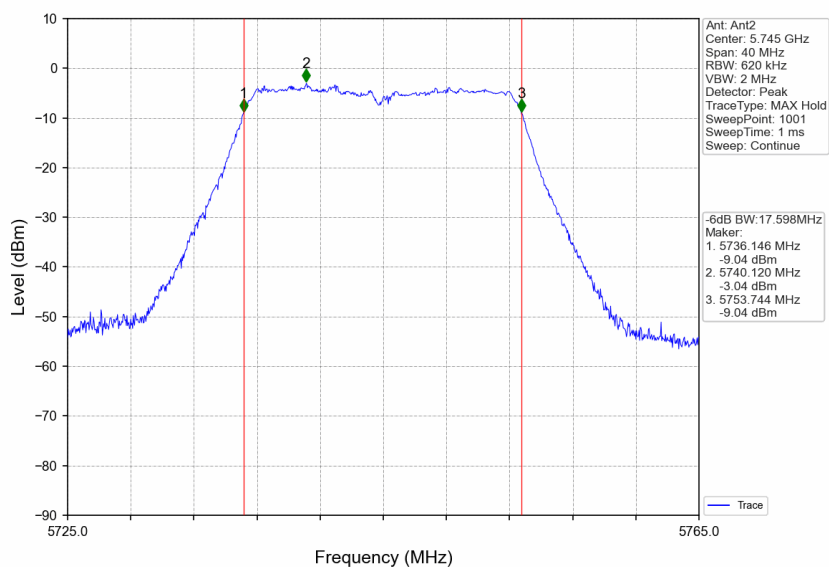
802.11n(HT20)_LCH_5745MHz_Ant2_NTNV
