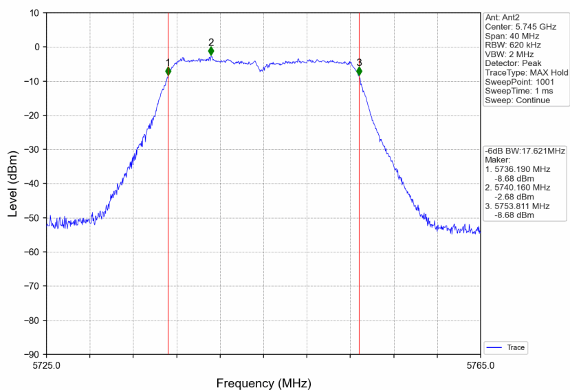
802.11ac(VHT20) LCH 5745MHz Ant2 NTNV
