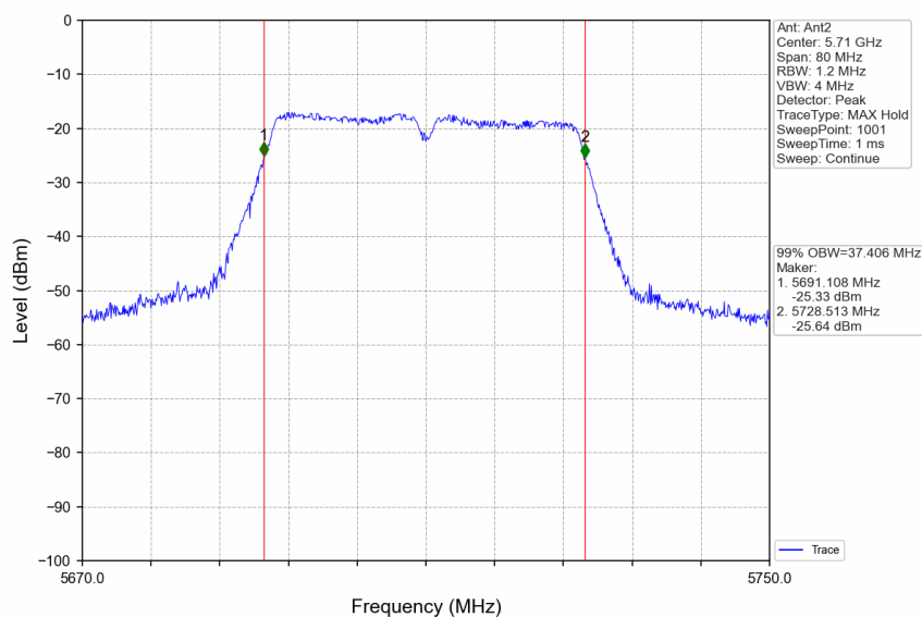
802.11ac(VHT40)_HCH_5710MHz_Ant2_NTNV
