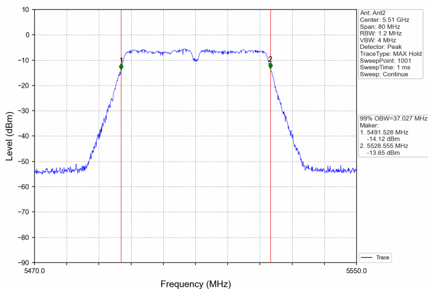
802.11ac(VHT40)_LCH_5510MHz_Ant2_NTNV
