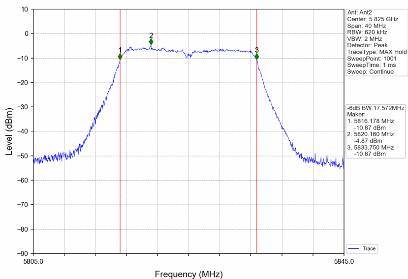
802.11ac(VHT20)_HCH_5825MHz_Ant2_NTNV
