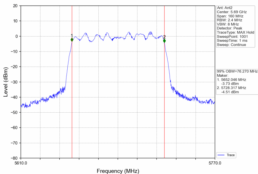
802.11ac(VHT80)_HCH_5690MHz_Ant2_NTNV
