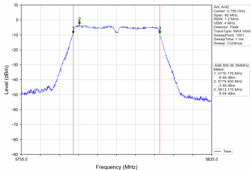
802.11ac(VHT40)_HCH_5795MHz_Ant2_NTNV
