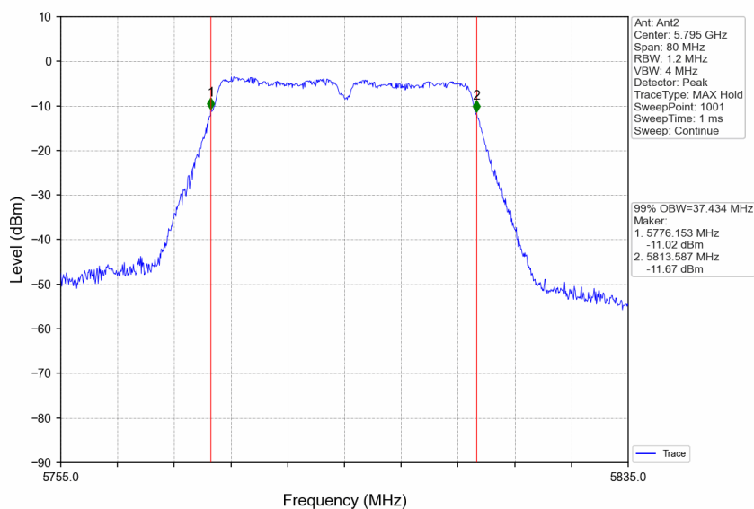
802.11ac(VHT40)_HCH_5795MHz_Ant2_NTNV
