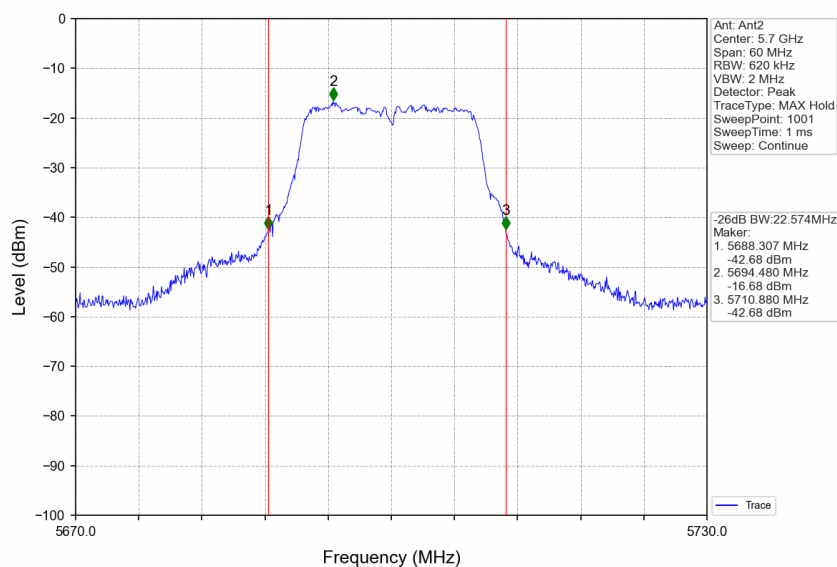
802.11ac(VHT20)_HCH_5700MHz_Ant2_NTNV
