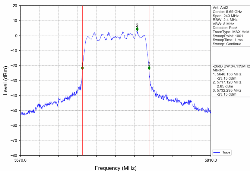
802.11ac(VHT80)_HCH_5690MHz_Ant2_NTNV
