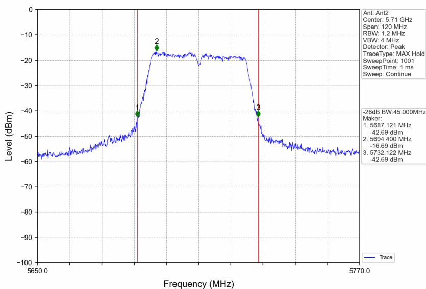
802.11ac(VHT40)_HCH_5710MHz_Ant2_NTNV
