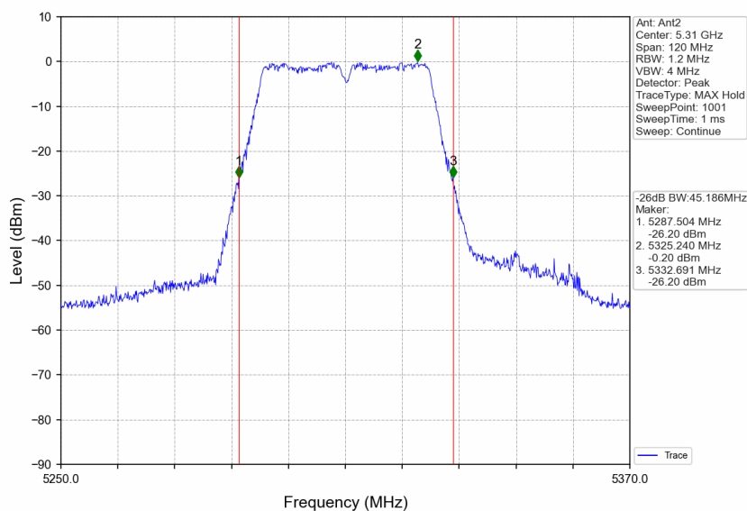
802.11ac(VHT40)_HCH_5310MHz_Ant2_NTNV
