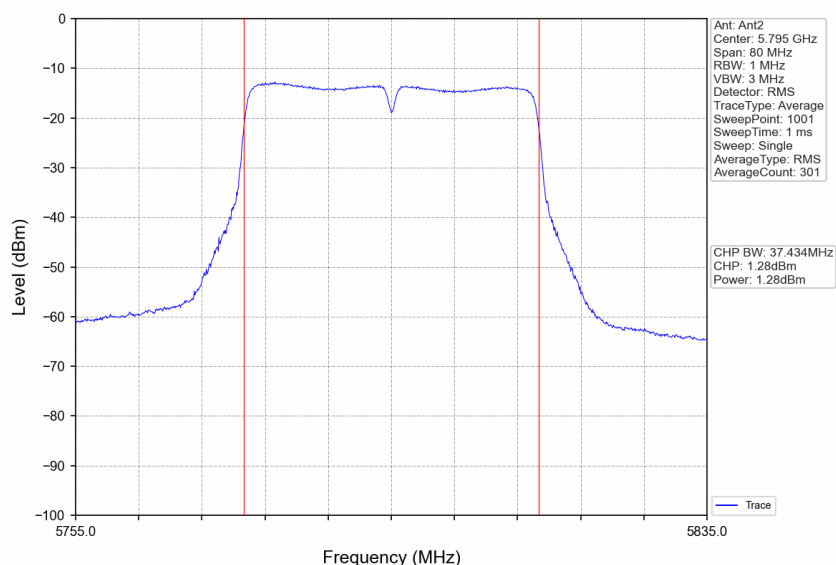
802.11ac(VHT40)_HCH_5795MHz_Ant2_NTNV
