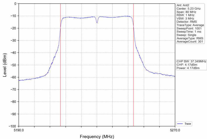
802.11ac(VHT40)_HCH_5230MHz_Ant2_NTNV
