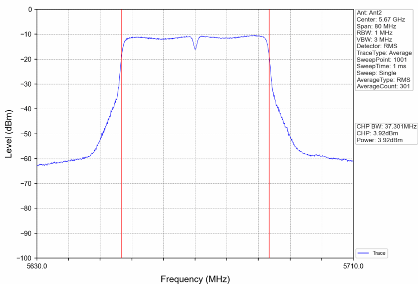
802.11ac(VHT40)_HCH_5670MHz_Ant2_NTNV
