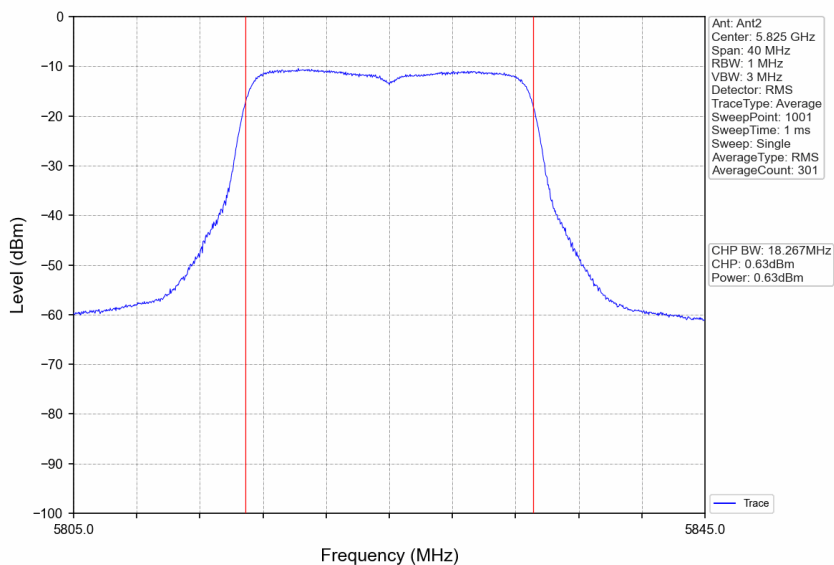
802.11ac(VHT20)_HCH_5825MHz_Ant2_NTNV
