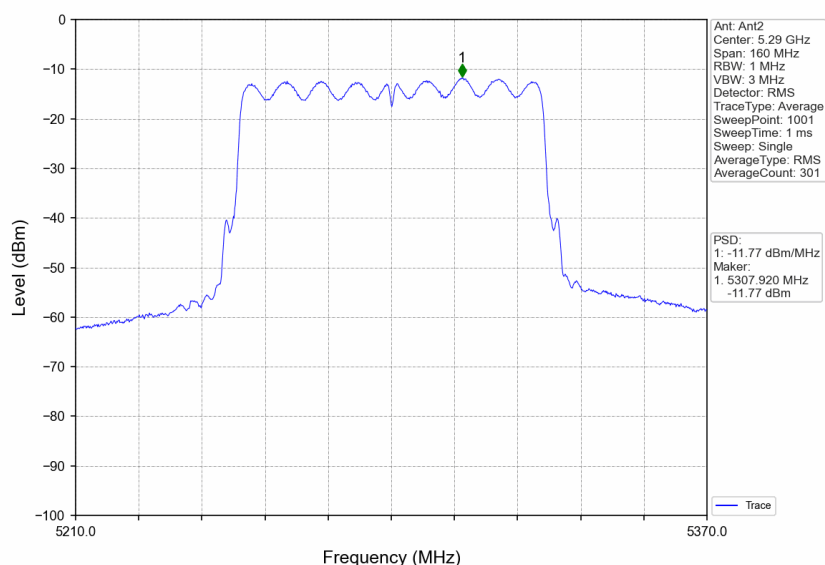
802.11ac(VHT80) MCH 5290MHz MIMO_NTNV
