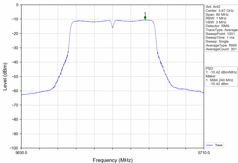
802.11ac(VHT40)_HCH_5670MHz_Ant2_NTNV
