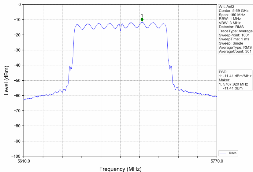
802.11ac(VHT80)_HCH_5690MHz_Ant2_NTNV
