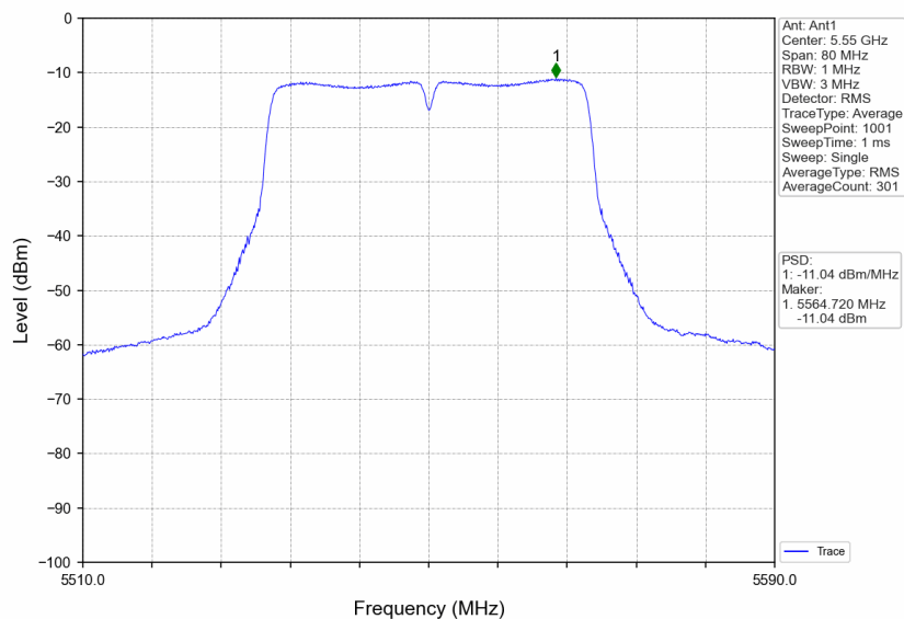
802.11ac(VHT40)_MCH_5550MHz_Ant1_NTNV
