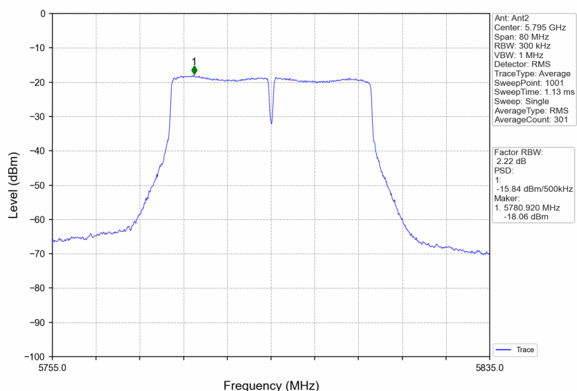
802.11ac(VHT40) HCH 5795MHz MIMO_NTNV
