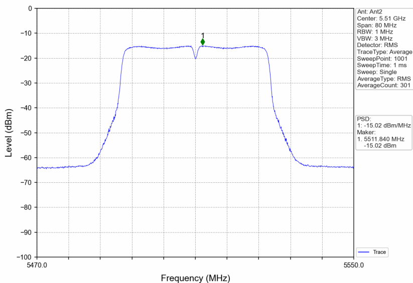
802.11ac(VHT40)_LCH_5510MHz_Ant2_NTNV
