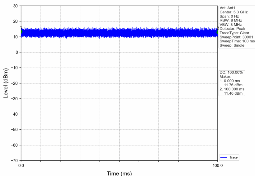
802.11n(HT20)_MCH_5300MHz_Ant1_NTNV
