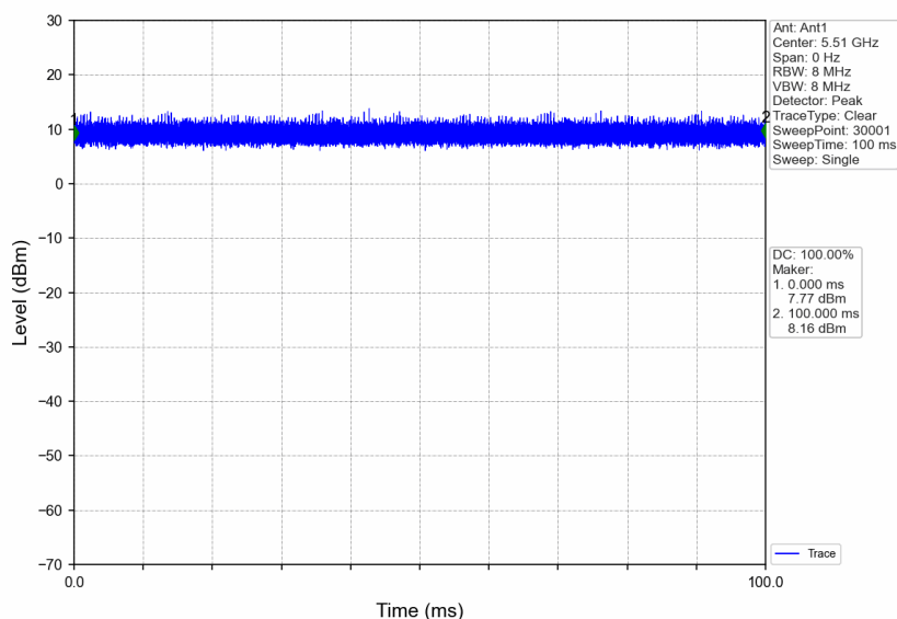
802.11ac(VHT40)_LCH_5510MHz_Ant1_NTNV
