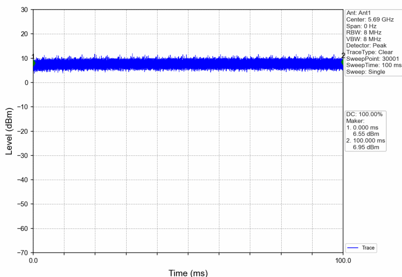
802.11ac(VHT80)_HCH_5690MHz_Ant1_NTNV
