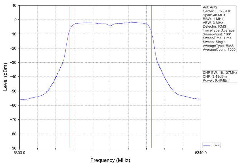
802.11ac(VHT20)_HCH_5320MHz_Ant2_NTNV
