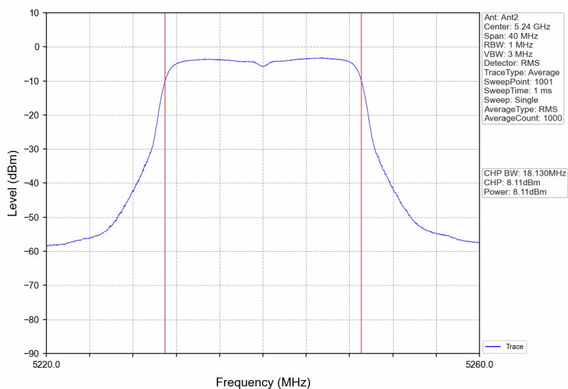
802.11ac(VHT20)_HCH_5240MHz_Ant2_NTNV
