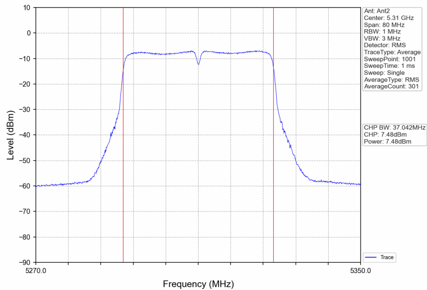
802.11ac(VHT40)_HCH_5310MHz_Ant2_NTNV
