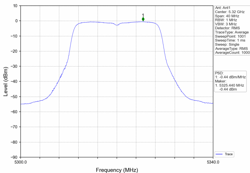
802.11ac(VHT20)_HCH_5320MHz_Ant1_NTNV
