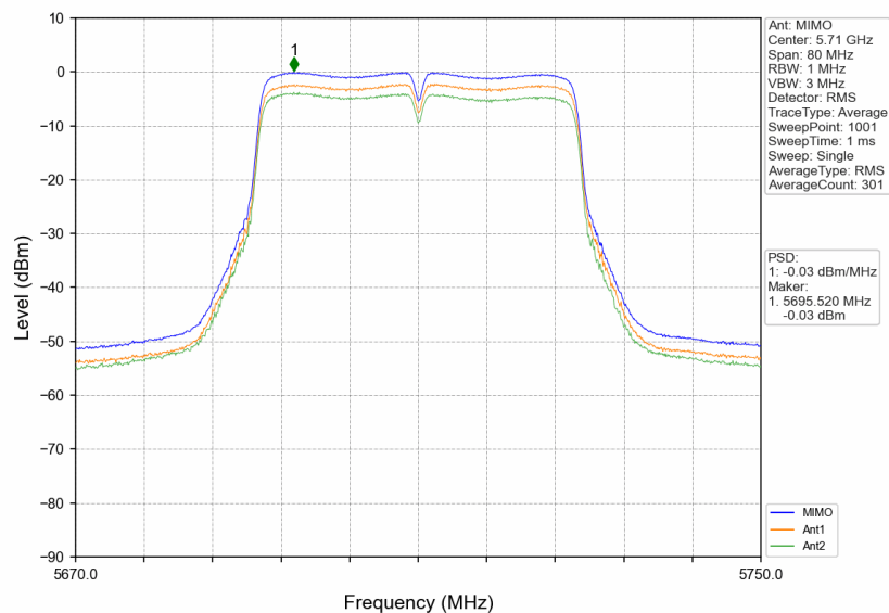
802.11n(HT40)_HCH_5710MHz_MIMO_NTNV
