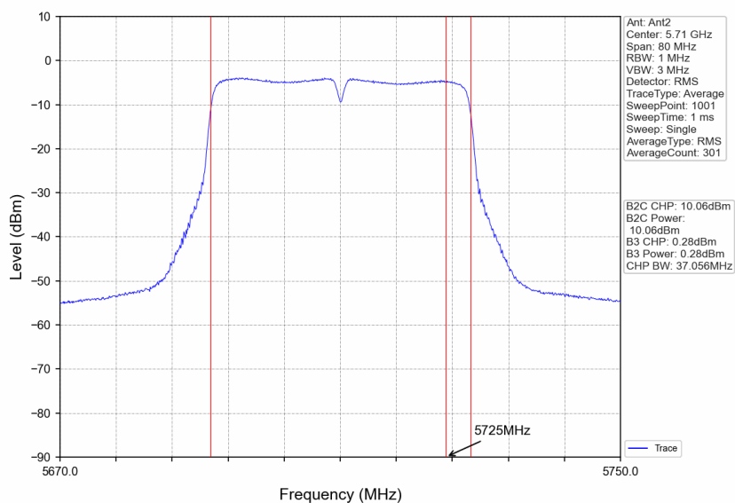
802.11ac(VHT40)_HCH_5710MHz_Ant2_NTNV
