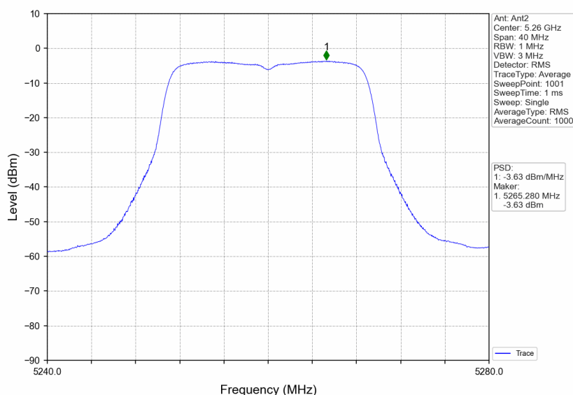
802.11n(HT20)_LCH_5260MHz_MIMO_NTNV
