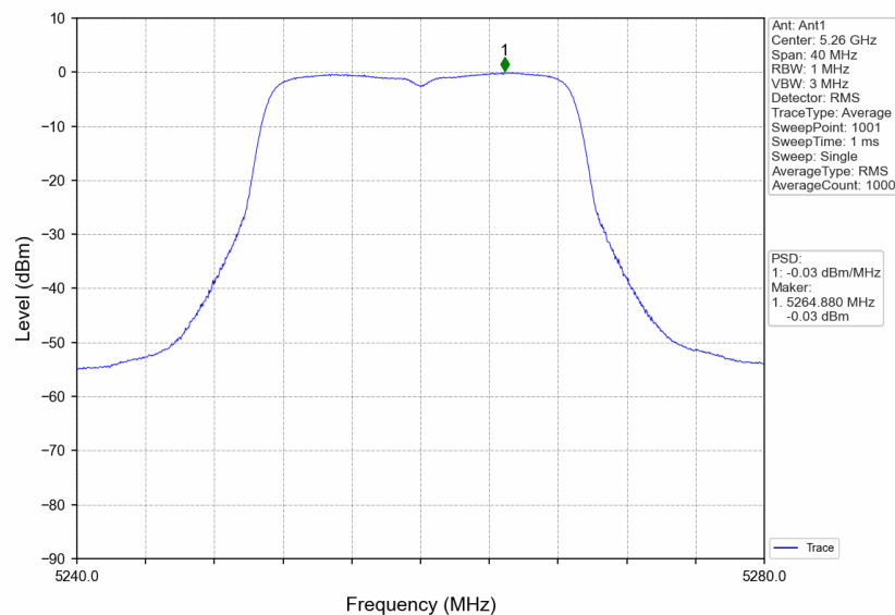
802.11ac(VHT20)_LCH_5260MHz_Ant1_NTNV
