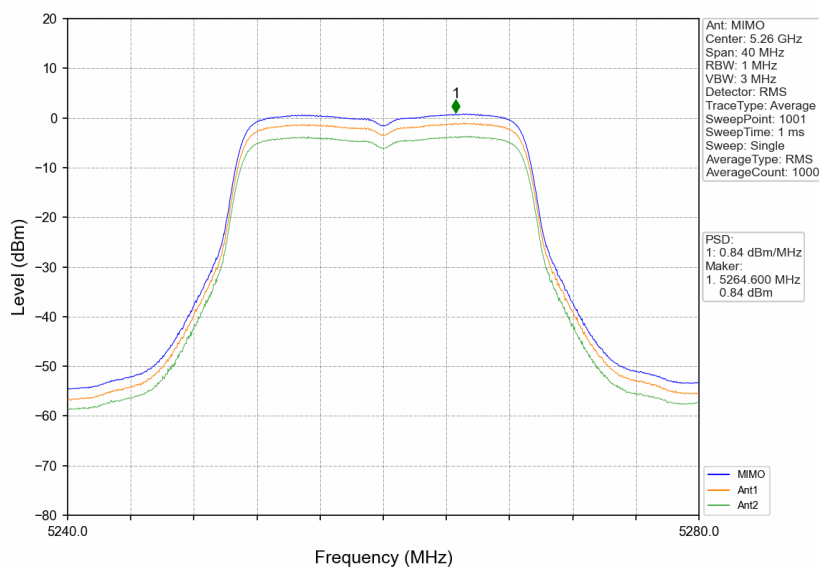
802.11n(HT20)_LCH_5260MHz_MIMO_NTNV
