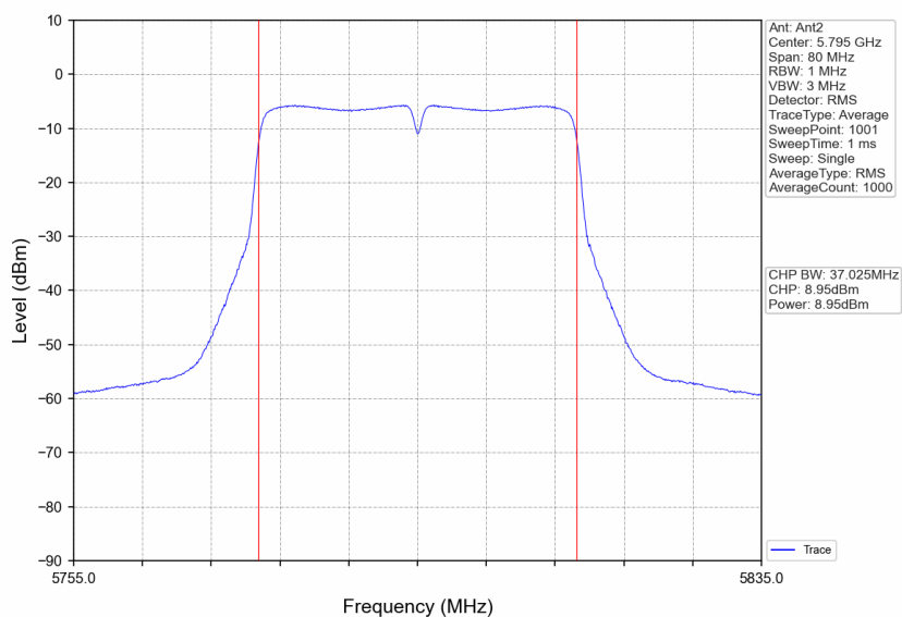
802.11ac(VHT40)_HCH_5795MHz_Ant2_NTNV
