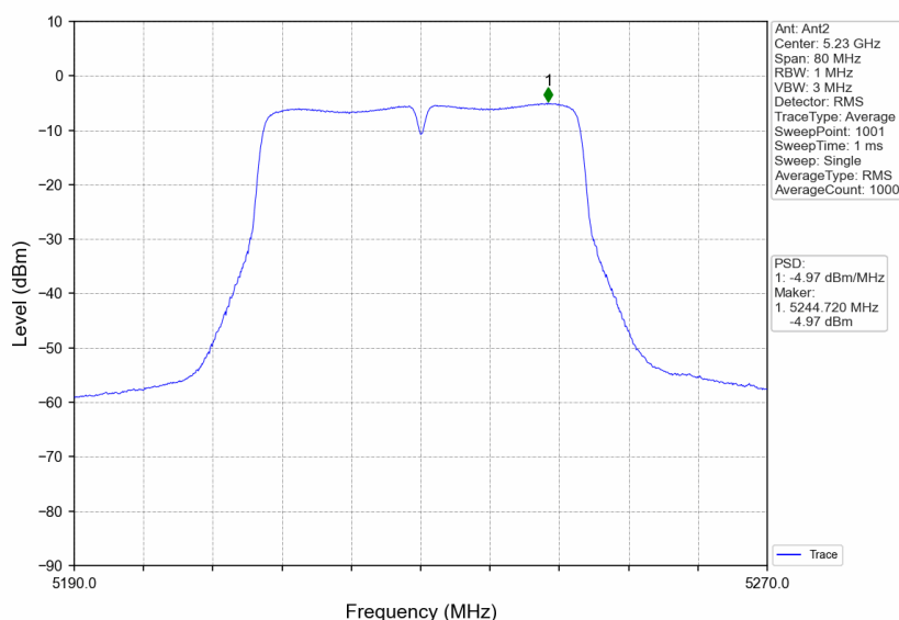
802.11n(HT40)_HCH_5230MHz_MIMO_NTNV
