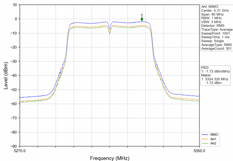
802.11n(HT40)_HCH_5310MHz_MIMO_NTNV
