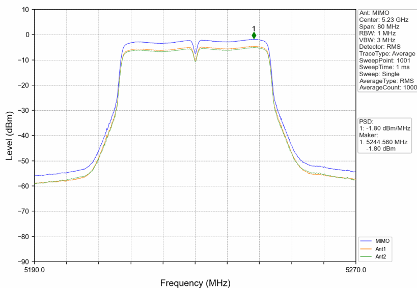
802.11n(HT40)_HCH_5230MHz_MIMO_NTNV
