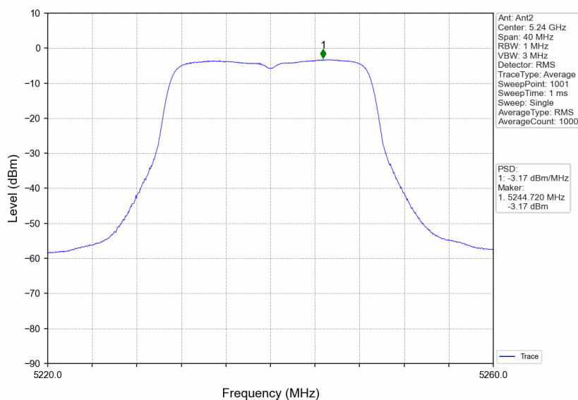
802.11ac(VHT20)_HCH_5240MHz_Ant2_NTNV
