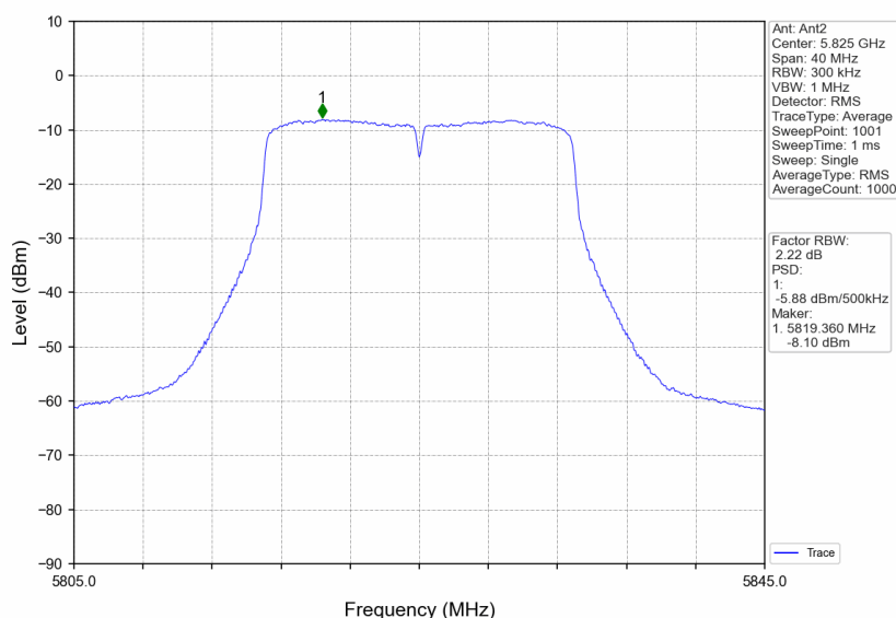
802.11ac(VHT20)_HCH_5825MHz_MIMO_NTNV
