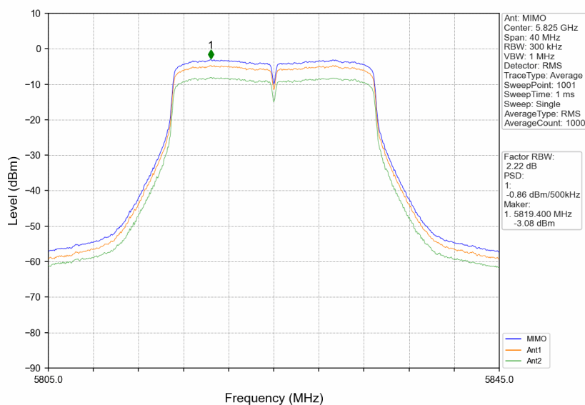
802.11ac(VHT20)_HCH_5825MHz_MIMO_NTNV
