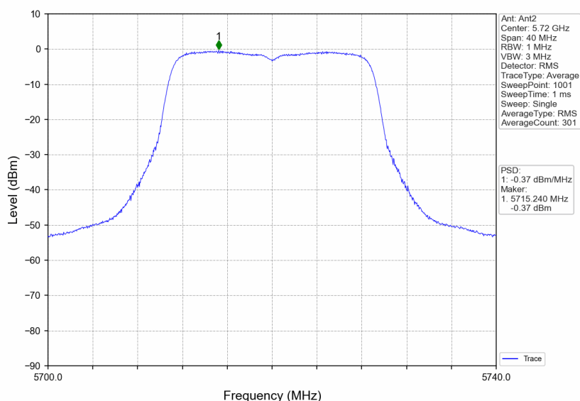
802.11ac(VHT20)_HCH_5720MHz_MIMO_NTNV
