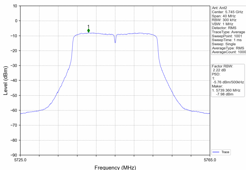
802.11ac(VHT20)_LCH_5745MHz_MIMO_NTNV
