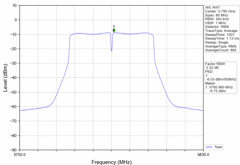
802.11ac(VHT40)_HCH_5795MHz_Ant1_NTNV
