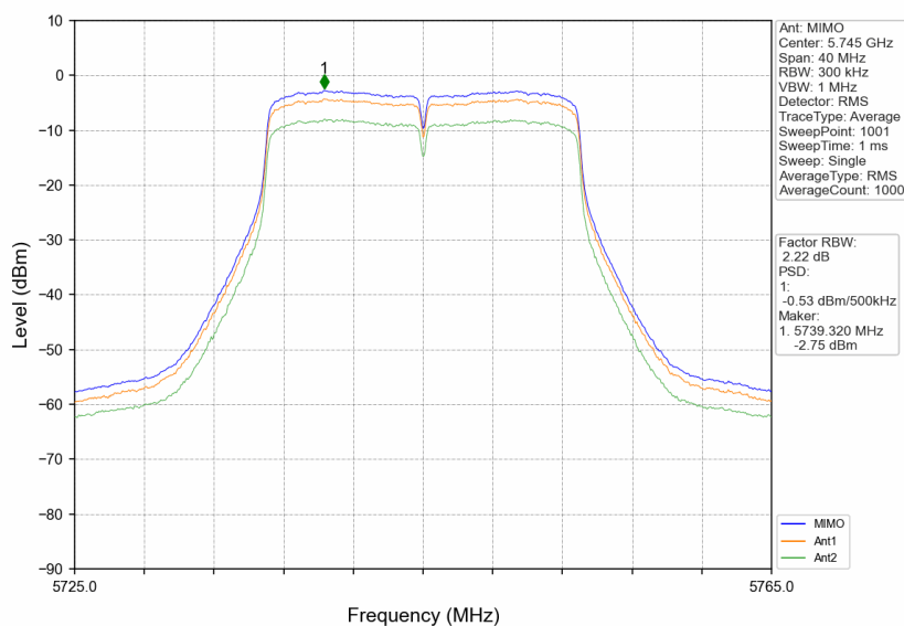
802.11ac(VHT20)_LCH_5745MHz_MIMO_NTNV
