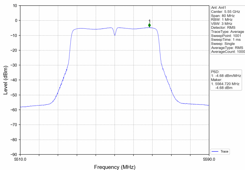
802.11ac(VHT40)_MCH_5550MHz_Ant1_NTNV
