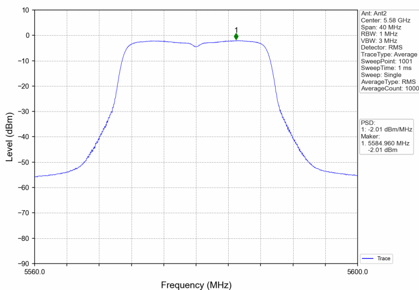
802.11ac(VHT20) MCH 5580MHz MIMO_NTNV
