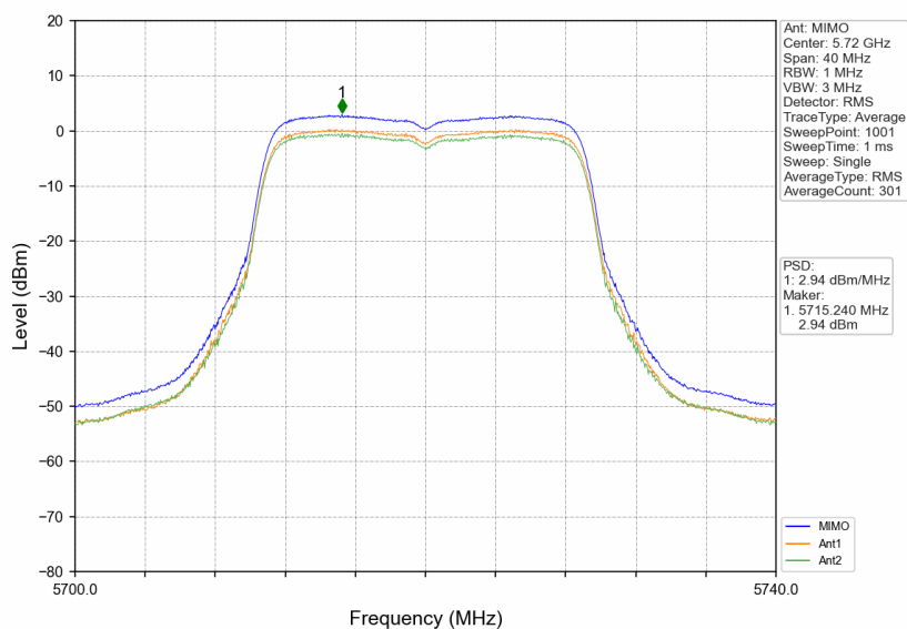
802.11ac(VHT20)_HCH_5720MHz_MIMO_NTNV
