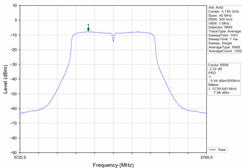
802.11n(HT20)_LCH_5745MHz_Ant2_NTNV
