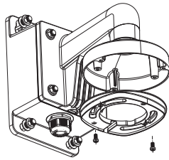
Figure 2-13 Fix the Adapter Plate
