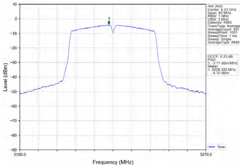
802.11n(HT40)_HCH_5230MHz_MIMO_NTNV
