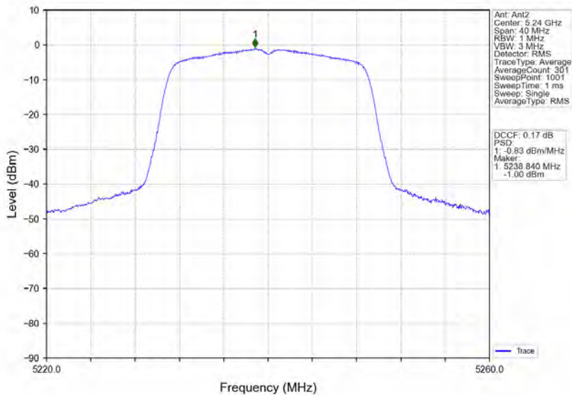
802.11ac(VHT20)_HCH_5240MHz_MIMO_NTNV
