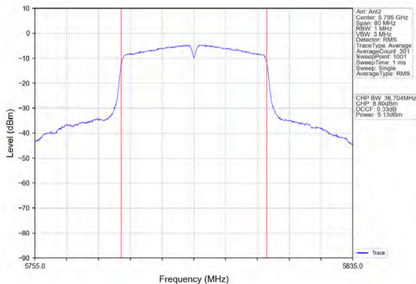
802.11ac(VHT40)_HCH_5795MHz_Ant2_NTNV
