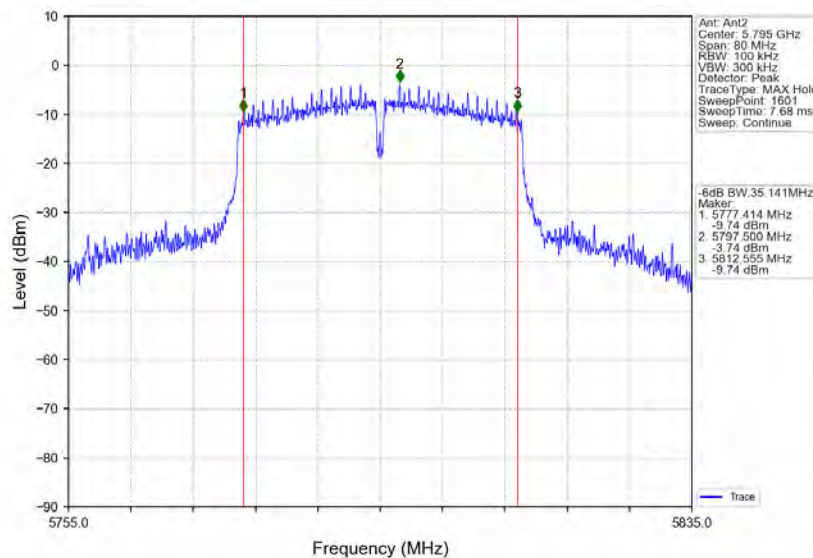
802.11ac(VHT40)_HCH_5795MHz_Ant2_NTNV
