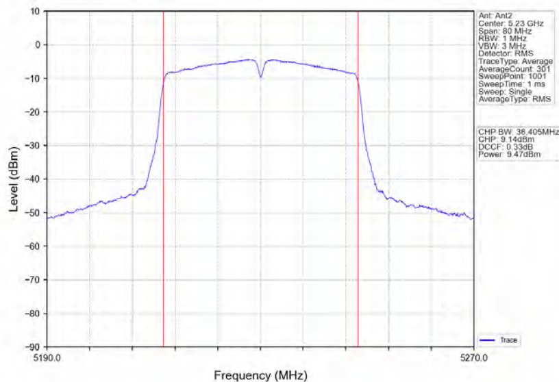
802.11ac(VHT40)_HCH_5230MHz_Ant2_NTNV
