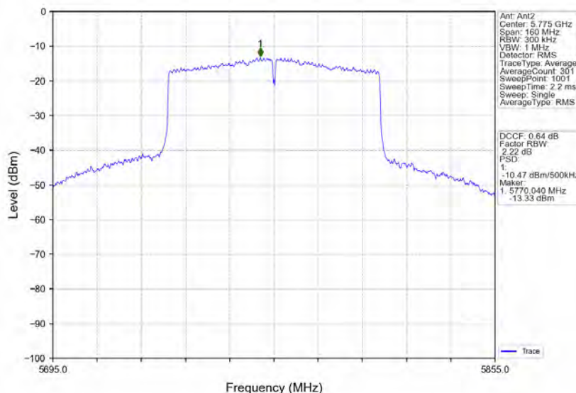
802.11ac(VHT80)_MCH_5775MHz_MIMO_NTNV
