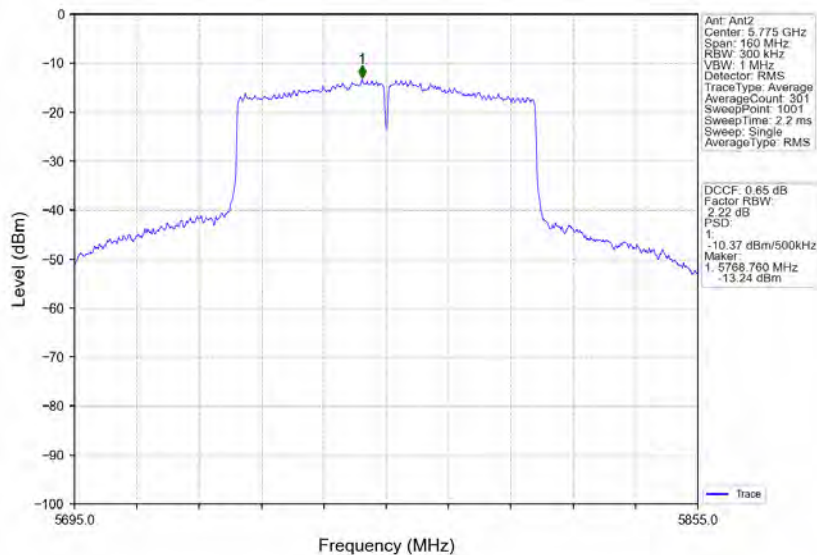
802.11ac(VHT80)_MCH_5775MHz_MIMO_NTNV
