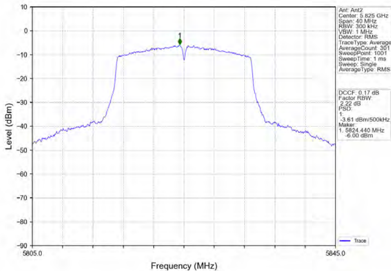
802.11ac(VHT20)_HCH_5825MHz_MIMO_NTNV
