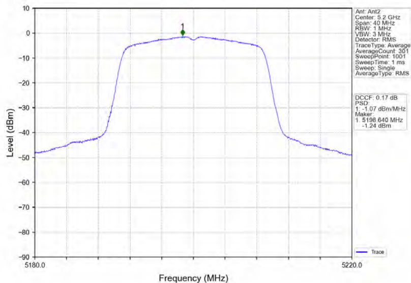
802.11ac(VHT20)_MCH_5200MHz_MIMO_NTNV
