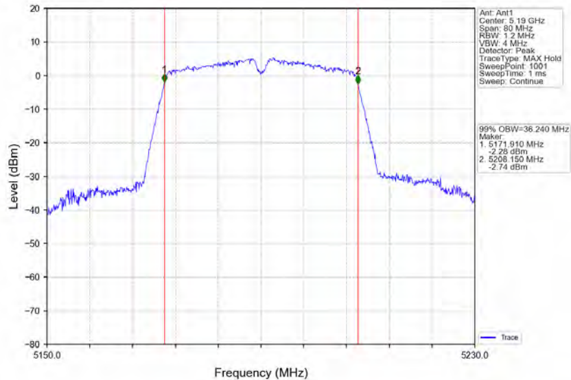
802.11ac(VHT40)_LCH_5190MHz_Ant4_NTNV
