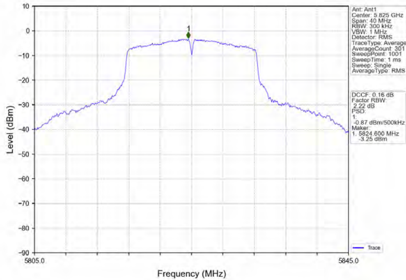
802.11a_HCH_5825MHz_Ant4_NTNV
