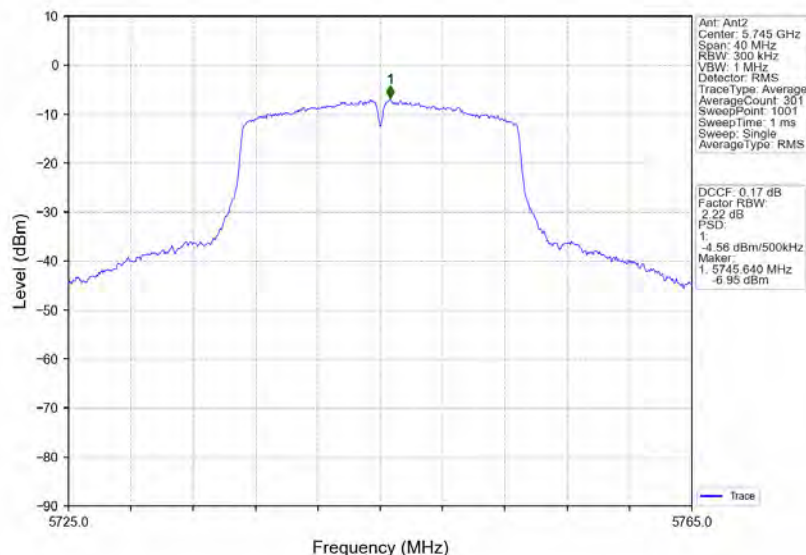
802.11n(HT20)_LCH_5745MHz_MIMO_NTNV
