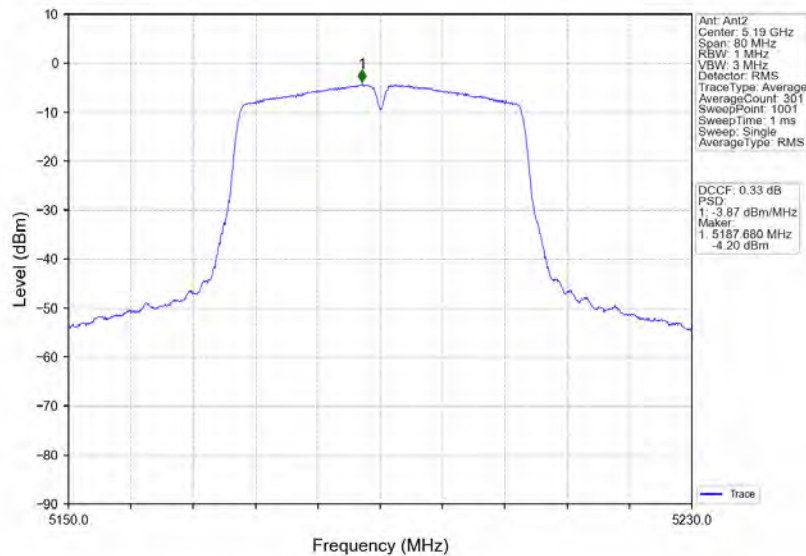
802.11n(HT40)_LCH_5190MHz_MIMO_NTNV
