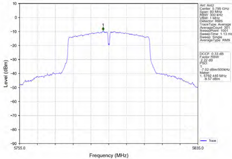
802.11ac(VHT40)_HCH_5795MHz_MIMO_NTNV
