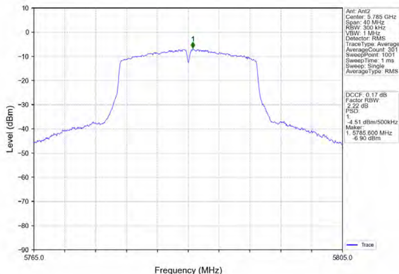
802.11ac(VHT20)_MCH_5785MHz_MIMO_NTNV
