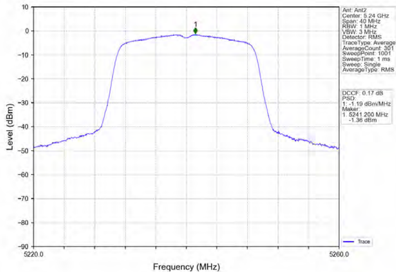
802.11ac(VHT20)_HCH_5240MHz_MIMO_NTNV
