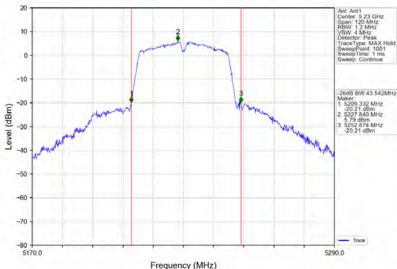
802.11ac(VHT40)_HCH_5230MHz_Ant4_NTNV
