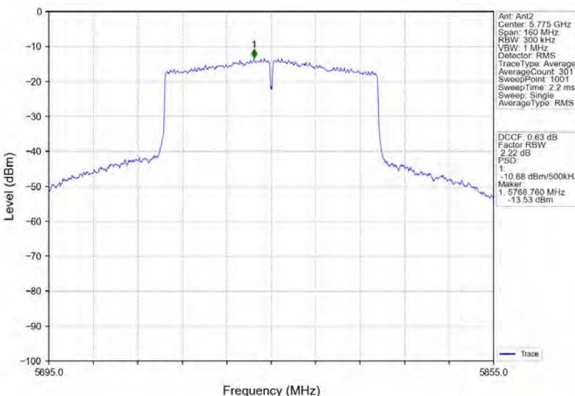
802.11ac(VHT80)_MCH_5775MHz_MIMO_NTNV
