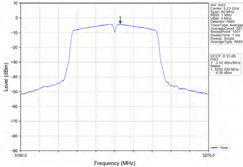
802.11ac(VHT40)_HCH_5230MHz_MIMO_NTNV
