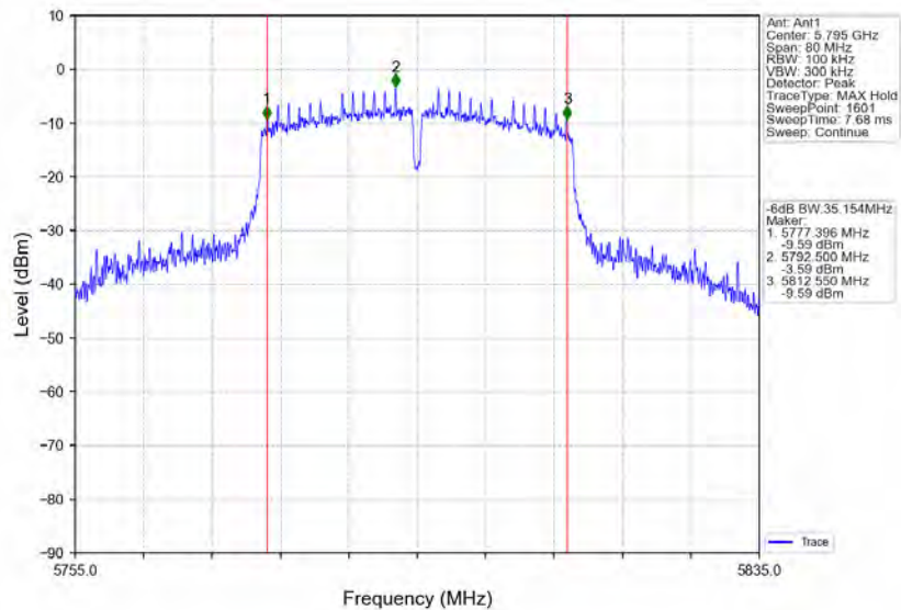
802.11ac(VHT40)_HCH_5795MHz_Ant4_NTNV
