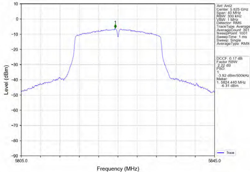
802.11ac(VHT20)_HCH_5825MHz_MIMO_NTNV
