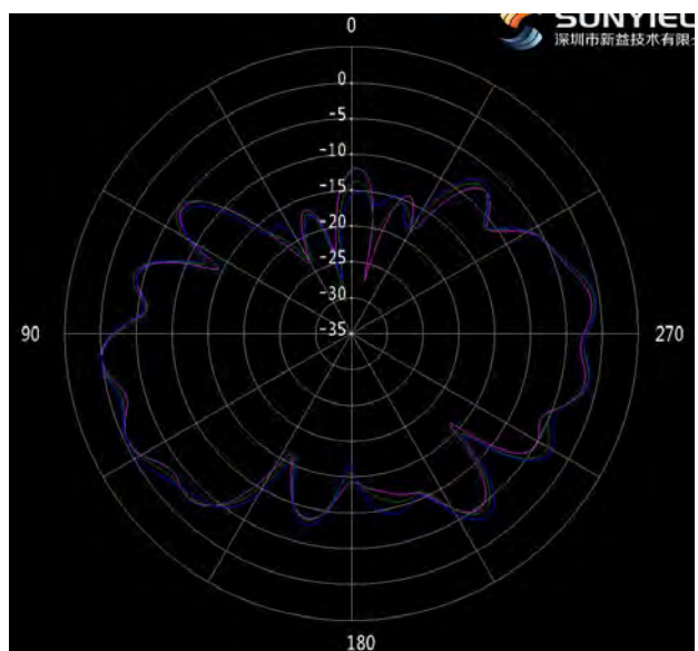
figure 13 ANT1 \theta=90^\circ (5.75/5.8/5.85GHz)
