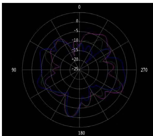
Figure 9. ANT1 \phi=90^\circ (5.15/5.2/5.25GHz)
