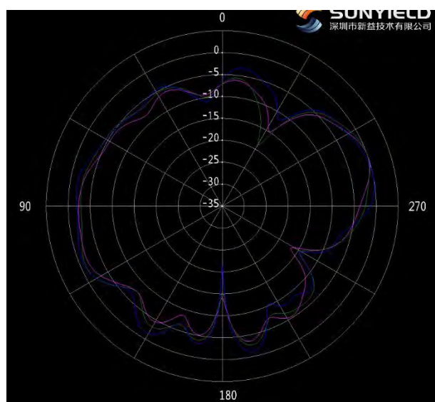
Figure 15 ANT2 \phi=90^\circ (2.4/2.45/2.5GHz)
