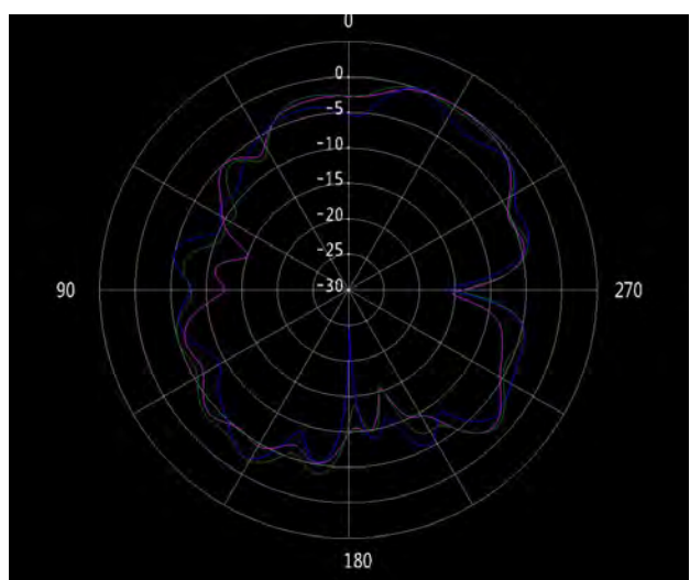
Figure 14 ANT2 \phi=0^\circ (2.4/2.45/2.5GHz)
