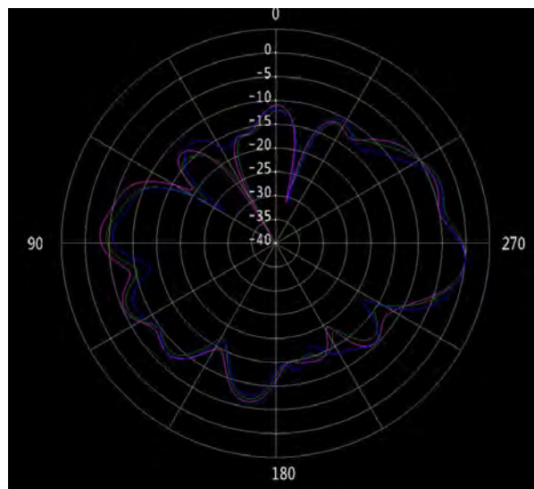
Figure 36 ANT4 \phi=90^\circ (5.15/5.2/5.25GHz)
