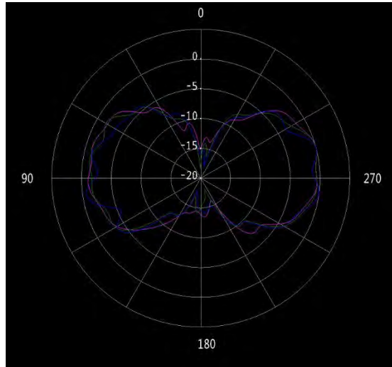
Figure 34 ANT4 \theta=90^\circ (2.4/2.45/2.5GHz)
