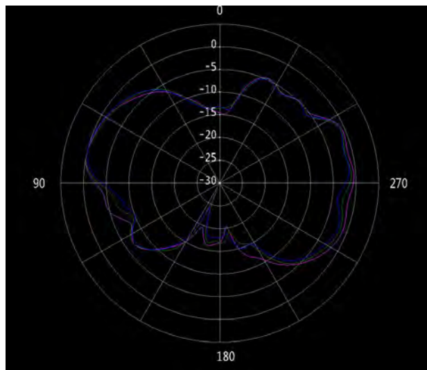
Figure 19 ANT2 theta=90° (5.15/5.2/5.25GHz)
