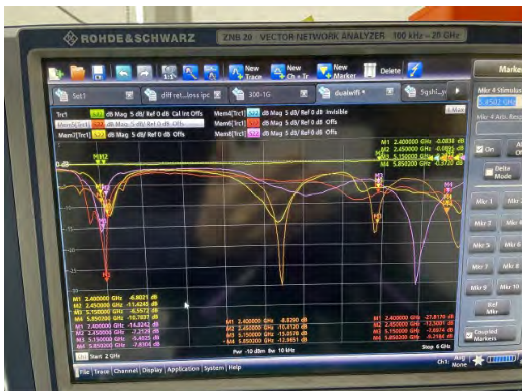
Figure 3.Return Loss
