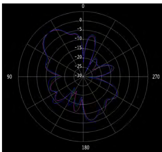
Figure 29 ANT3 phi=0° (5.75/5.8/5.85GHz)
