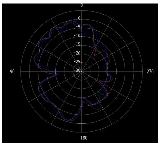
Figure 5. ANT1 \phi=0^\circ (2.4/2.45/2.5GHz)
