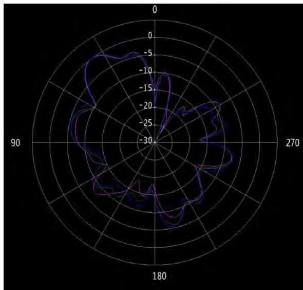
Figure 26 ANT3 \phi=0^\circ (5.15/5.2/5.25GHz)
