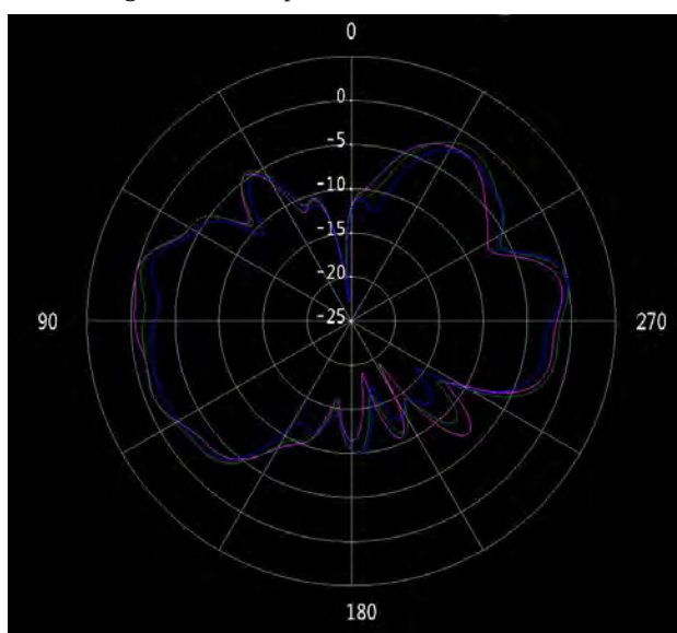
Figure 21 ANT2 phi=90° (5.75/5.8/5.85GHz)
