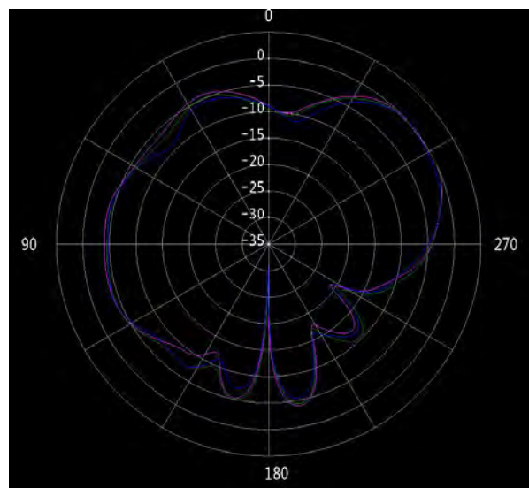
Figure 42 ANT5 (BT) \phi=90^\circ (2.4/2.45/2.5GHz)
