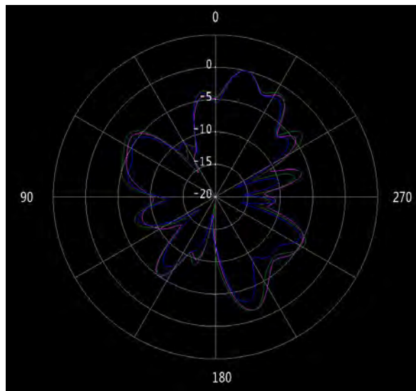
Figure 32 ANT4 \phi=0^\circ (2.4/2.45/2.5GHz)
