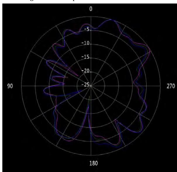
Figure 18 ANT2 phi=90° (5.15/5.2/5.25GHz)
