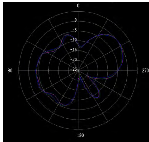
Figure 33 ANT4 \phi=90^\circ (2.4/2.45/2.5GHz)
