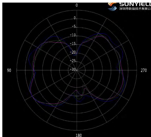
Figure 16 ANT2 theta=90° (2.4/2.45/2.5GHz)
