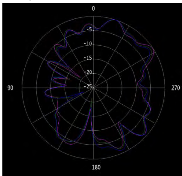
Figure 17 ANT2 phi=0° (5.15/5.2/5.25GHz)
