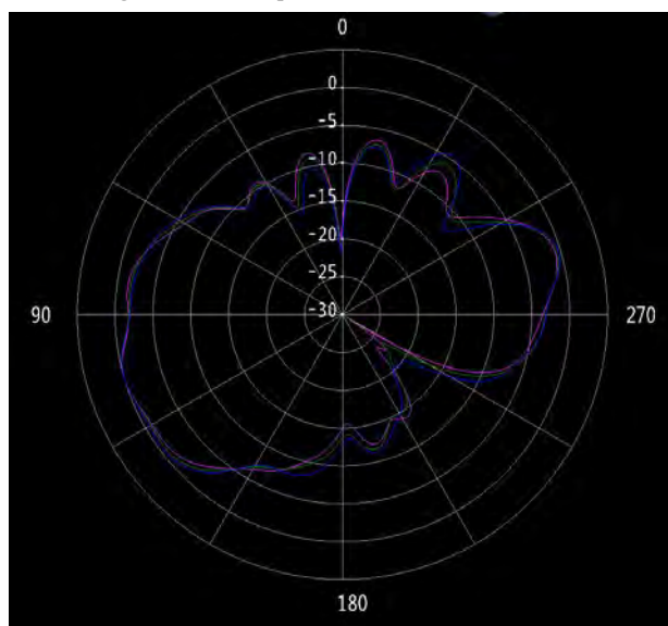
Figure 30 ANT3 phi=90° (5.75/5.8/5.85GHz)
