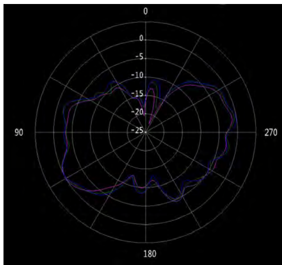
Figure 28 ANT3 theta=90° (5.15/5.2/5.25GHz)
