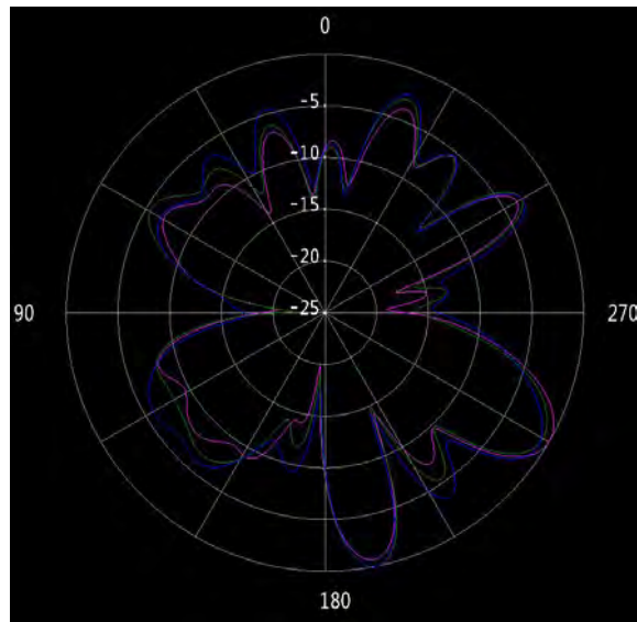
Figure 35 ANT4 \phi=0^\circ (5.15/5.2/5.25GHz)
