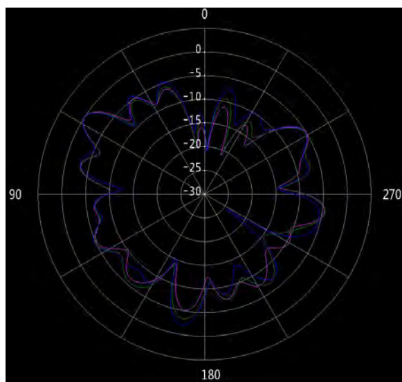
Figure 8. ANT1 \phi=0^\circ (5.15/5.2/5.25GHz)
