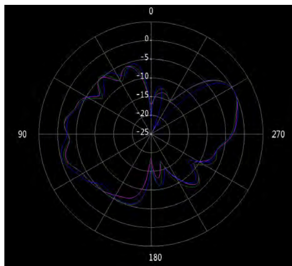
Figure 27 ANT3 \phi=90^\circ (5.15/5.2/5.25GHz)
