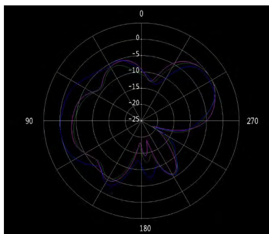
Figure 6. ANT1 \phi=90^\circ (2.4/2.45/2.5GHz)
