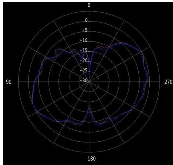
Figure 31 ANT3 \theta=90^\circ (5.75/5.8/5.85GHz)
