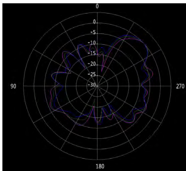
Figure 20 ANT2 phi=0° (5.75/5.8/5.85GHz)
