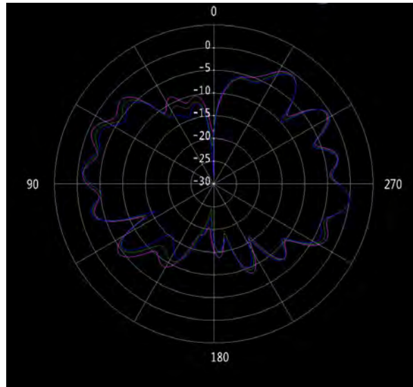
Figure 40 ANT4 \theta=90^\circ (5.75/5.8/5.85GHz)
