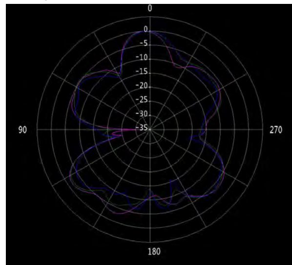
Figure 41 ANT5 (BT) \phi=0^\circ (2.4/2.45/2.5GHz)
