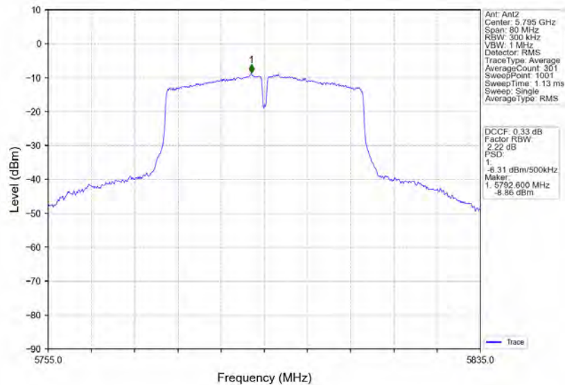
802.11ac(VHT40)_HCH_5795MHz_MIMO_NTNV
