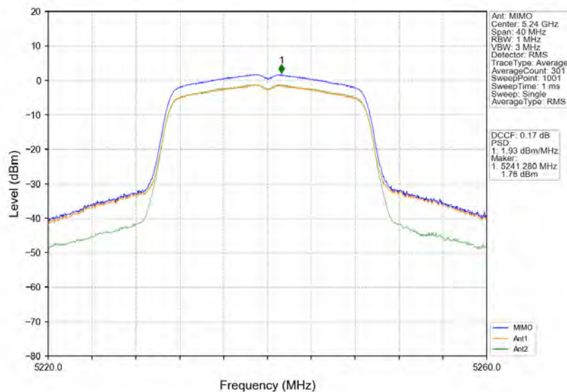
802.11ac(VHT20)_HCH_5240MHz_MIMO_NTNV
