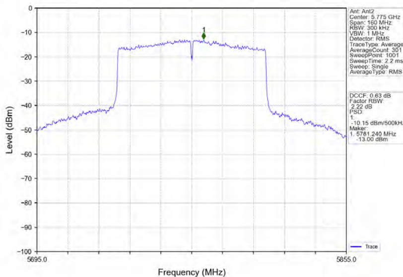
802.11ac(VHT80)_MCH_5775MHz_Ant2_NTNV
