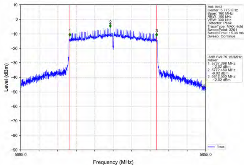
802.11ac(VHT80)_MCH_5775MHz_Ant2_NTNV
