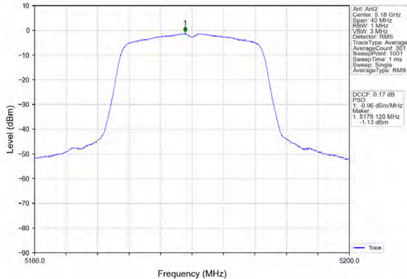
802.11ac(VHT20)_LCH_5180MHz_MIMO_NTNV
