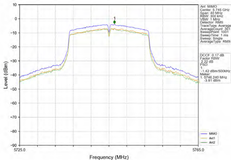
802.11ac(VHT20)_LCH_5745MHz_MIMO_NTNV
