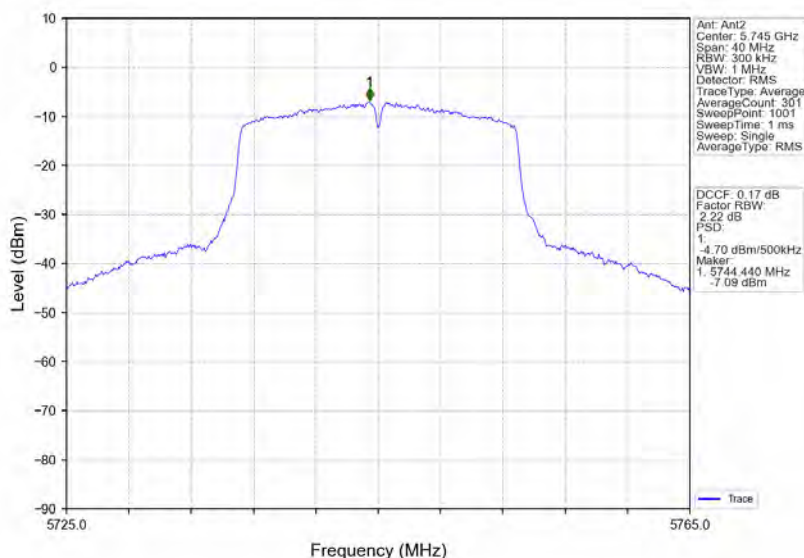
802.11n(HT20)_LCH_5745MHz_Ant2_NTNV
