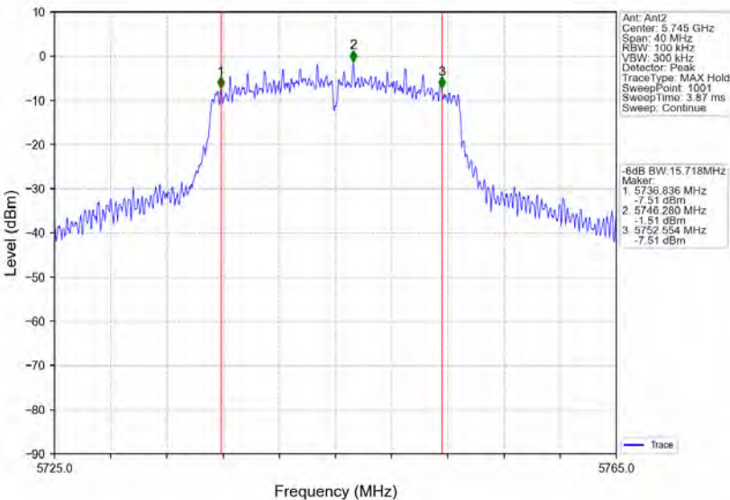
802.11n(HT20)_LCH_5745MHz_Ant2_NTNV
