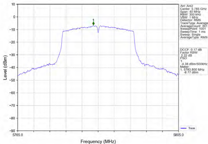
802.11ac(VHT20)_MCH_5785MHz_Ant2_NTNV
