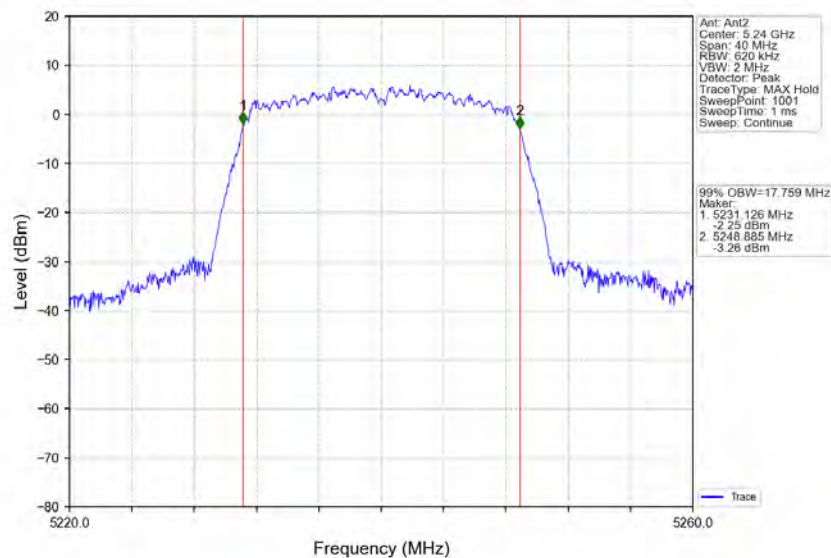
802.11n(HT20)_HCH_5240MHz_Ant2_NTNV
