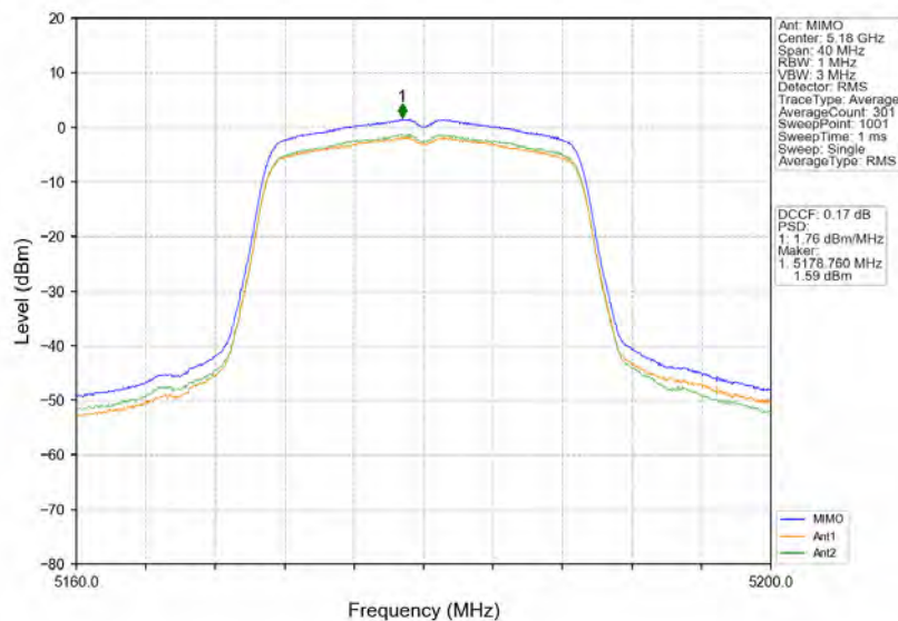
802.11ac(VHT20)_LCH_5180MHz_MIMO_NTNV
