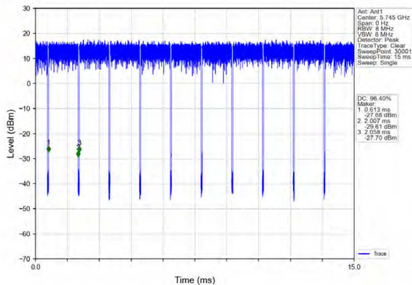
802.11a_LCH_5745MHz_Ant1_NTNV
