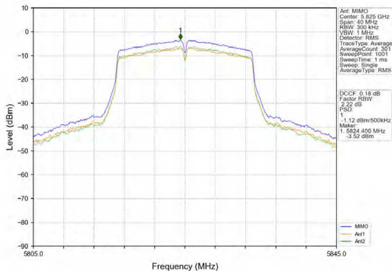
802.11ac(VHT20)_HCH_5825MHz_MIMO_NTNV
