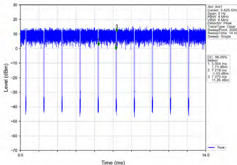
802.11ac(VHT20)_HCH_5825MHz_Ant1_NTNV
