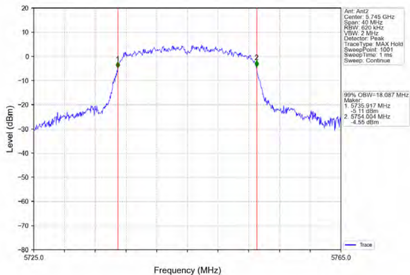
802.11ac(VHT20)_LCH_5745MHz_Ant2_NTNV
