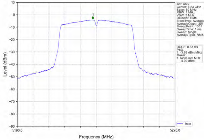
802.11ac(VHT40)_HCH_5230MHz_MIMO_NTNV
