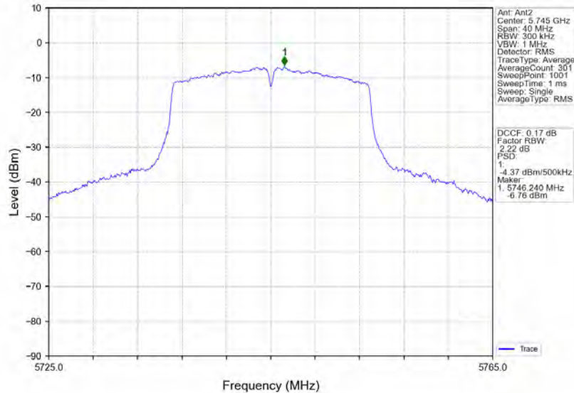
802.11ac(VHT20)_LCH_5745MHz_MIMO_NTNV
