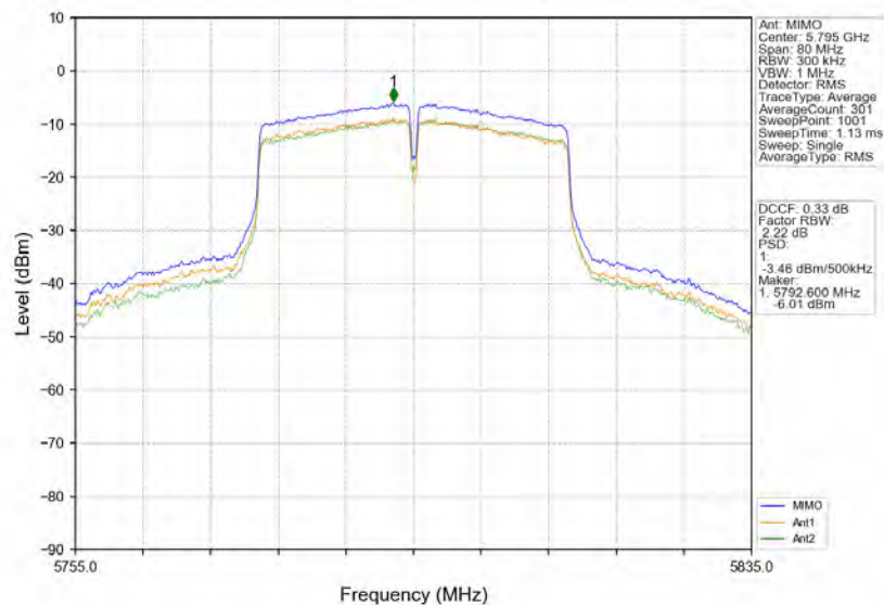
802.11ac(VHT40)_HCH_5795MHz_MIMO_NTNV
