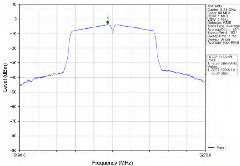
802.11ac(VHT40)_HCH_5230MHz_MIMO_NTNV
