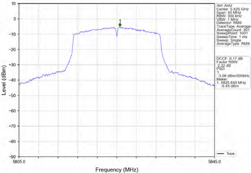
802.11ac(VHT20)_HCH_5825MHz_MIMO_NTNV
