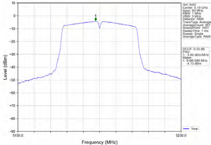
802.11n(HT40)_LCH_5190MHz_MIMO_NTNV
