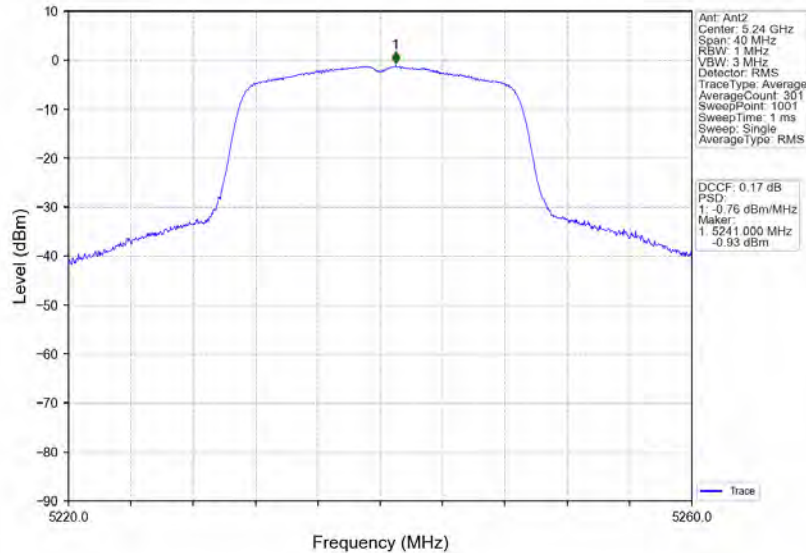
802.11ac(VHT20)_HCH_5240MHz_MIMO_NTNV
