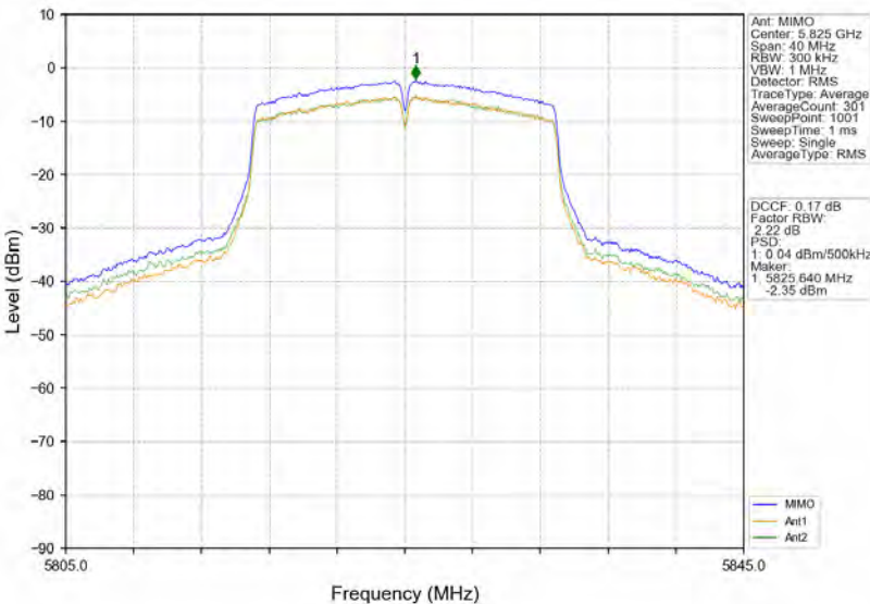
802.11ac(VHT20)_HCH_5825MHz_MIMO_NTNV
