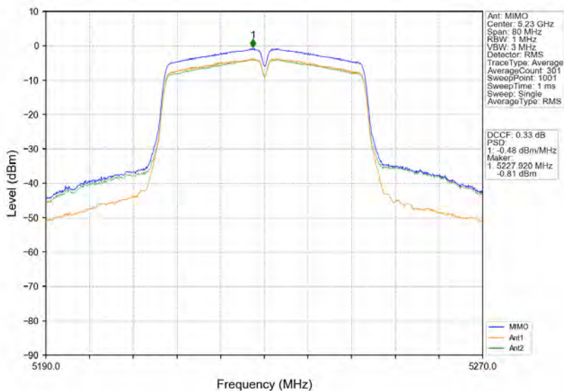
802.11ac(VHT40)_HCH_5230MHz_MIMO_NTNV
