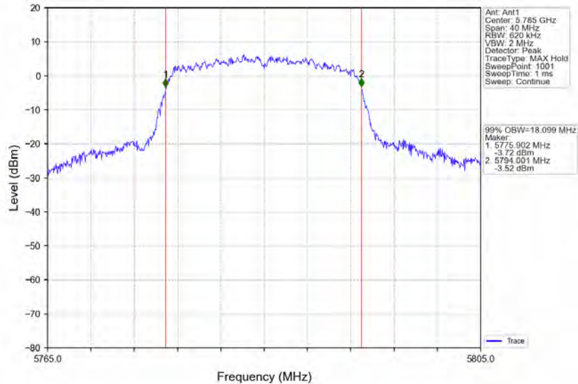
802.11ac(VHT20)_MCH_5785MHz_Ant4_NTNV
