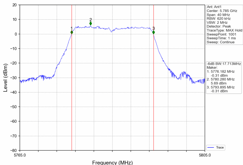
802.11ac(VHT20)_MCH_5785MHz_Ant1_NTNV
