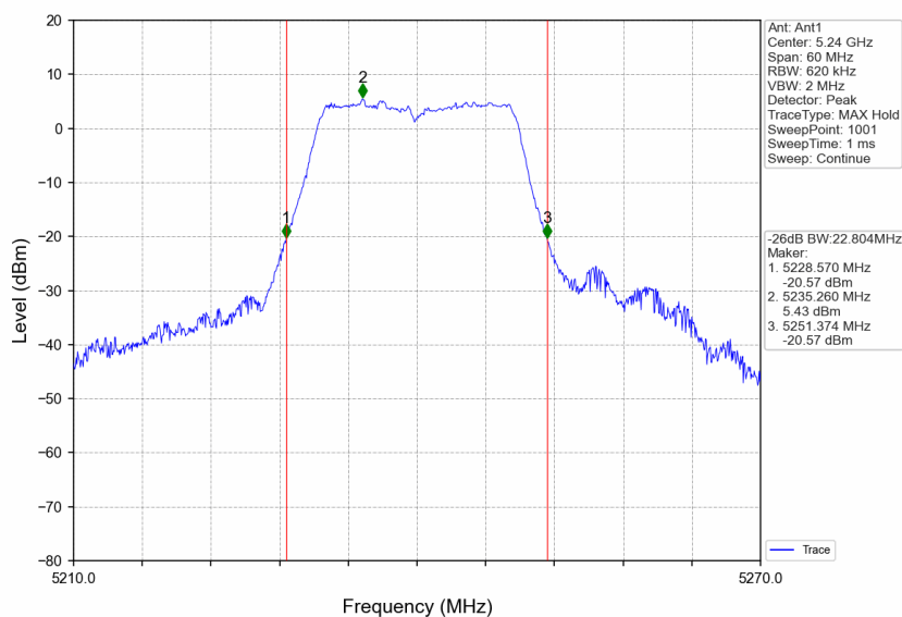
802.11n(HT20)_HCH_5240MHz_Ant1_NTNV
