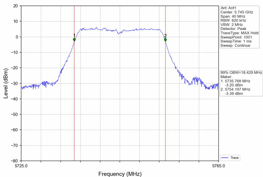
802.11ac(VHT20)_LCH_5745MHz_Ant1_NTNV
