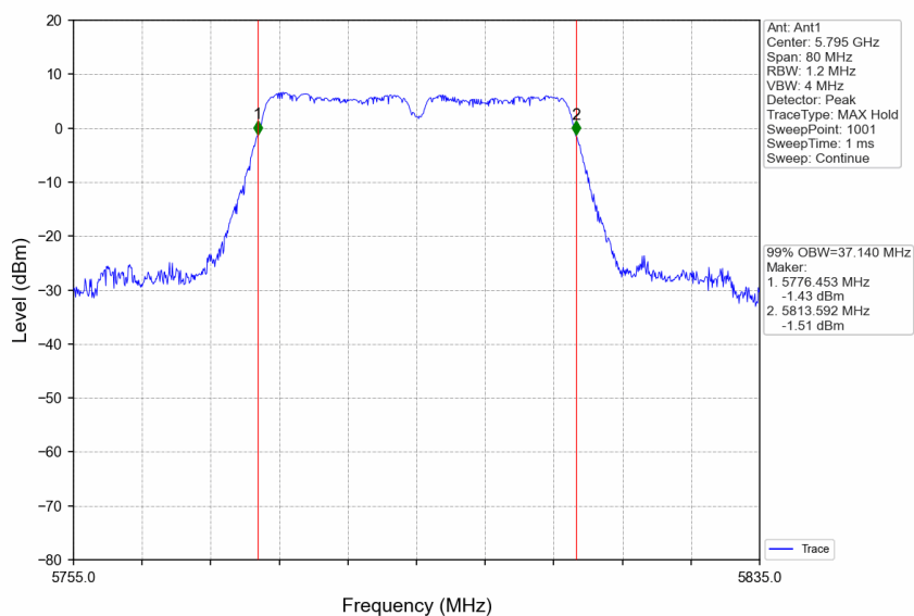
802.11ac(VHT40)_HCH_5795MHz_Ant1_NTNV
