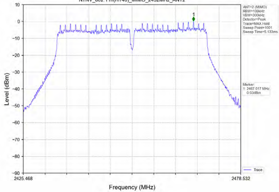
Unwanted Emissions in Non-restricted Frequency Bands NTNV_802.11n(HT40)_MIMO_2452MHz_ANT2
