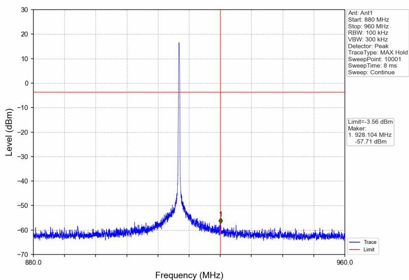
FSK_HCH_917.4MHz_Ant1_NTNV
