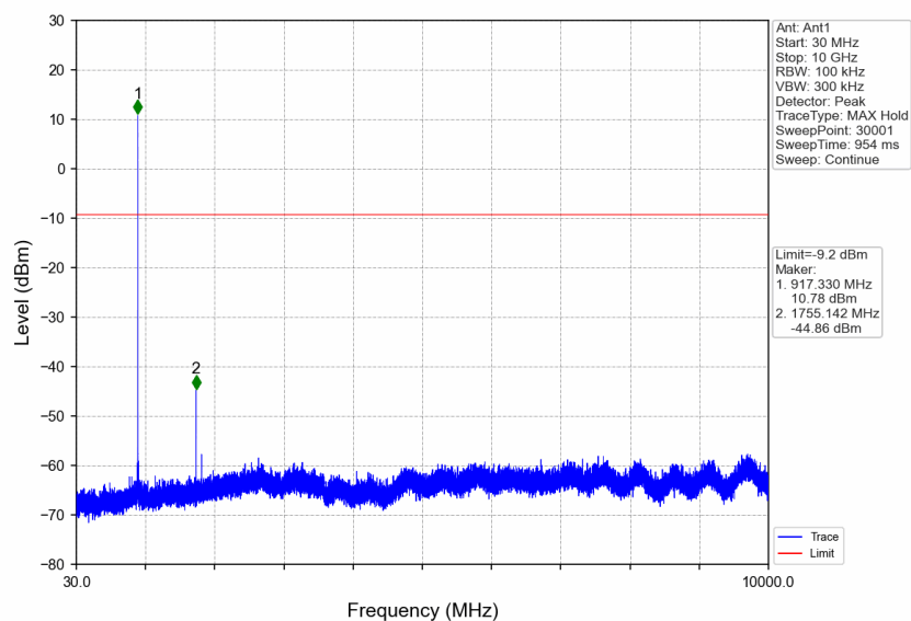
FSK_HCH_917.4MHz_Ant1_NTNV
