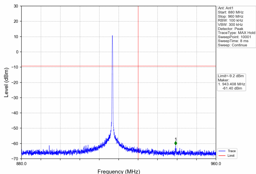
FSK_HCH_917.4MHz_Ant1_NTNV
