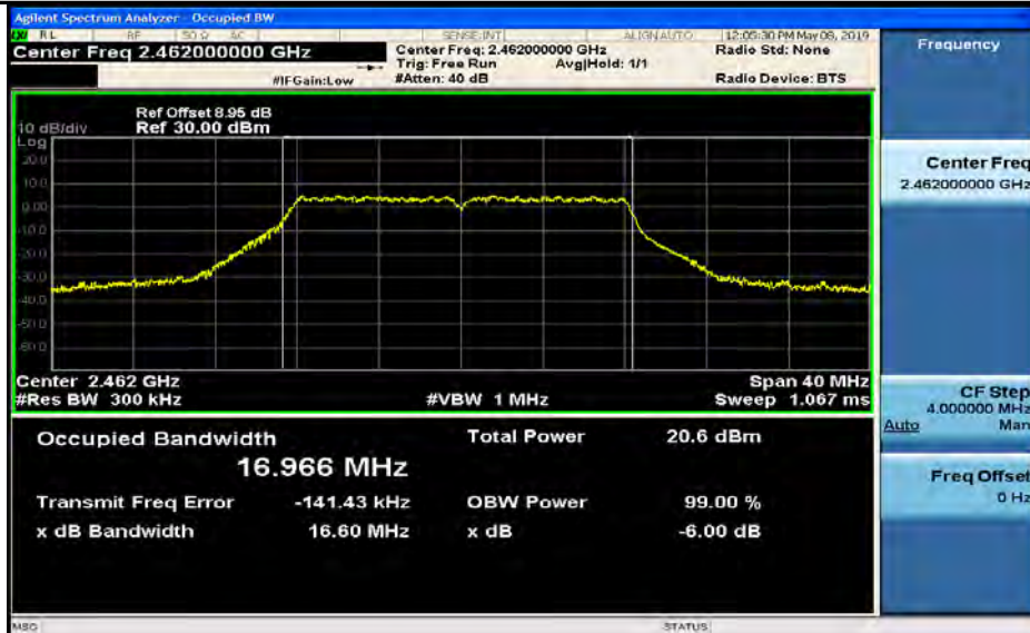
Occupied Bandwidth_11N20SISO_2462_Ant1
