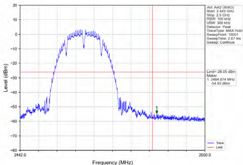
802.11b_HCH_2462MHz_Ant2 (SISO)_NTN
