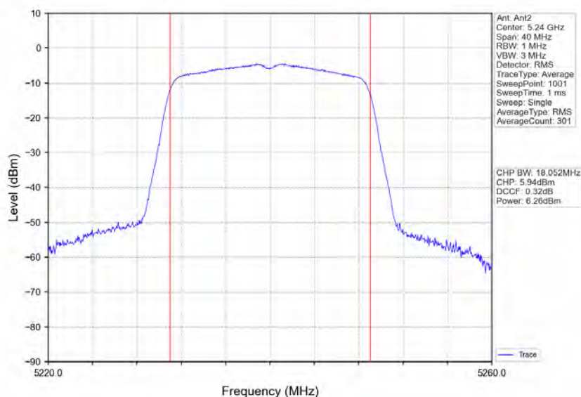
802.11n(HT20)_HCH_5240MHz_Ant2_NTNV
