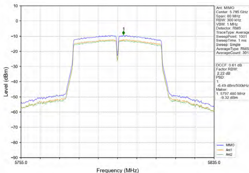
802.11ac(VHT40)_HCH_5795MHz_MIMO_NTNV
