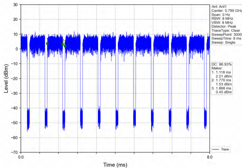
802.11ac(VHT40)_HCH_5795MHz_Ant1_NTN
