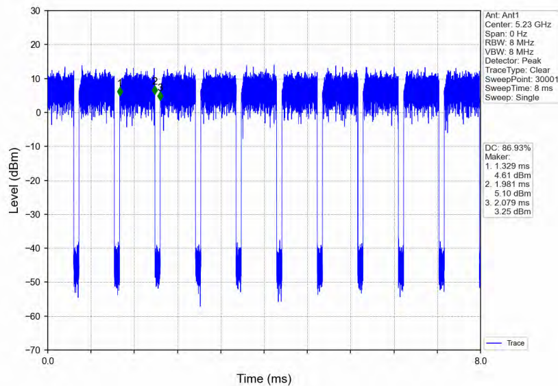
802.11ac(VHT40)_HCH_5230MHz_Ant1_NTN
