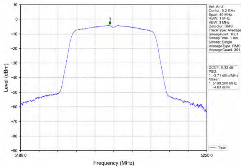
802.11ac(VHT20)_MCH_5200MHz_Ant2_NTNV
