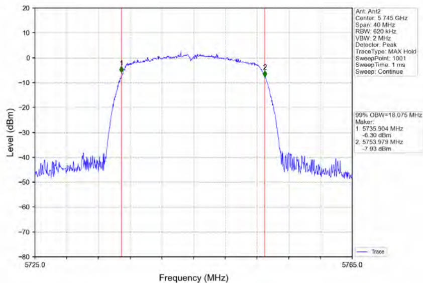
802.11ac(VHT20)_LCH_5745MHz_Ant2_NTNV
