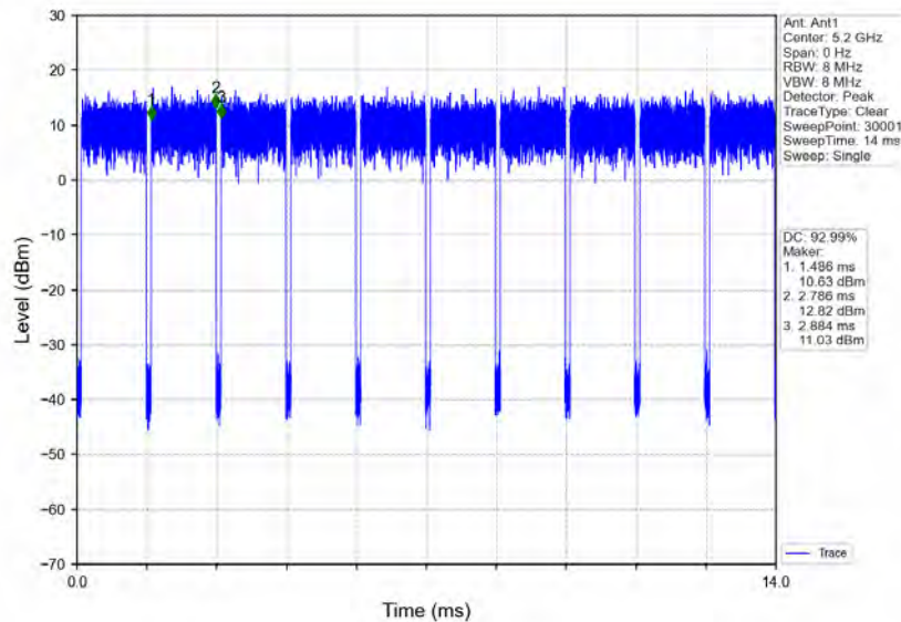
802.11n(HT20)_MCH_5200MHz_Ant1_NTN
