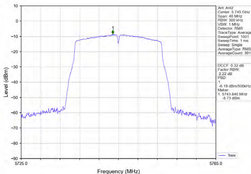
802.11n(HT20)_LCH_5745MHz_Ant2_NTNV
