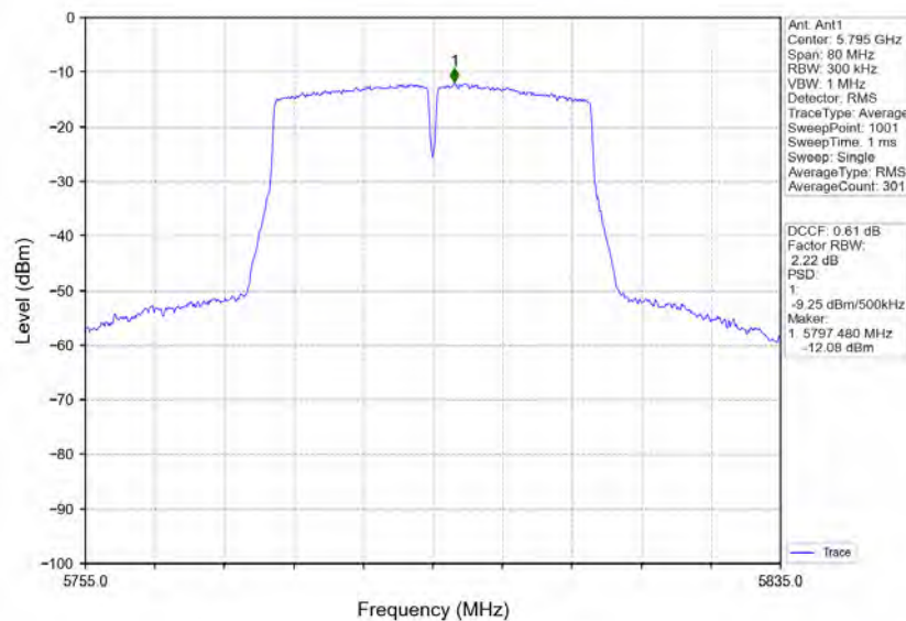
802.11ac(VHT40)_HCH_5795MHz_Ant1_NTN
