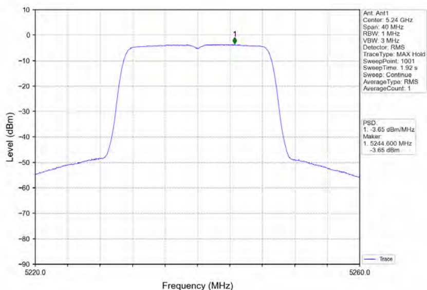
802.11ac(VHT20)_HCH 5240MHz_Ant1_NTN
