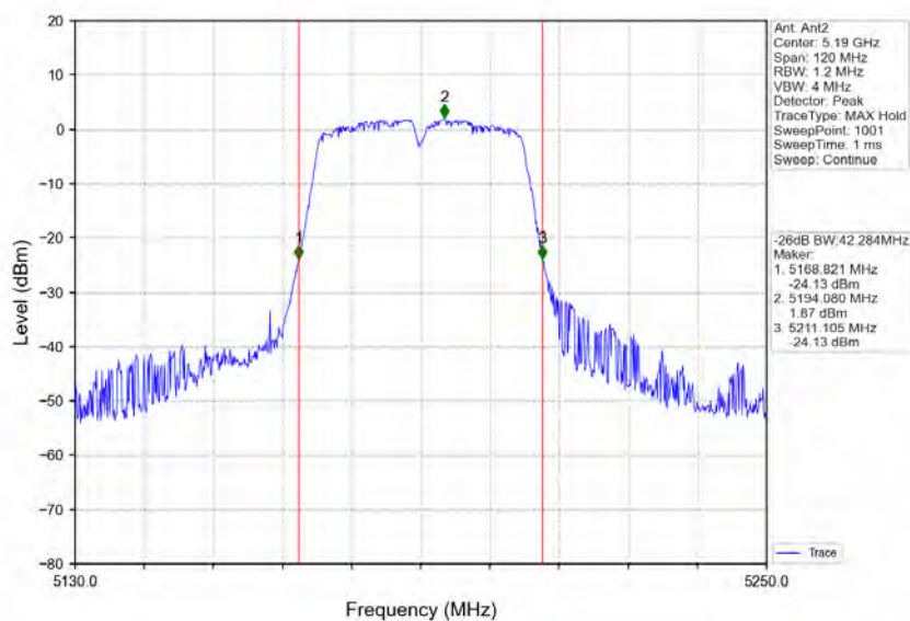
802.11ac(VHT40)_LCH_5190MHz_Ant2_NTNV
