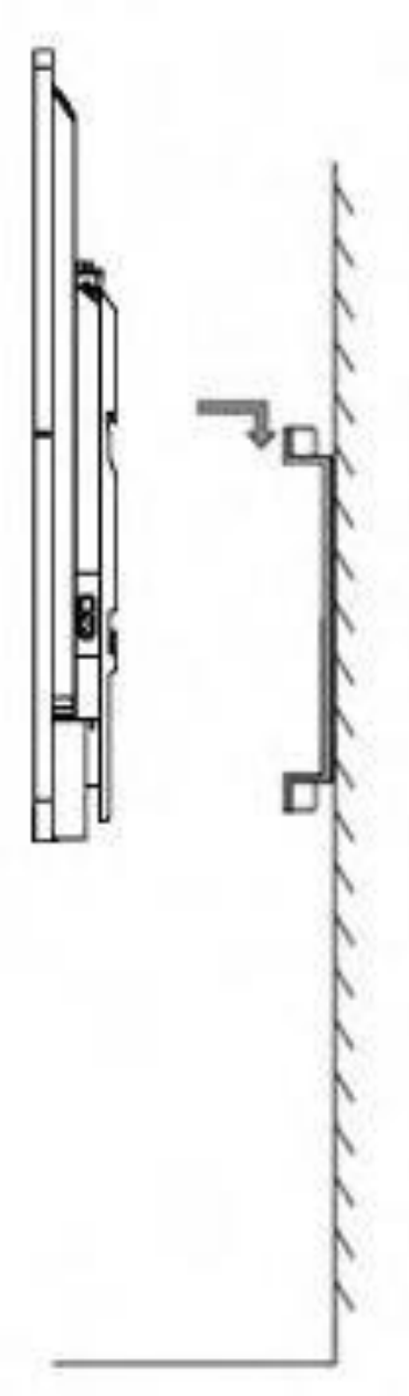
Figure 3-5 Wall Mounting Side View
