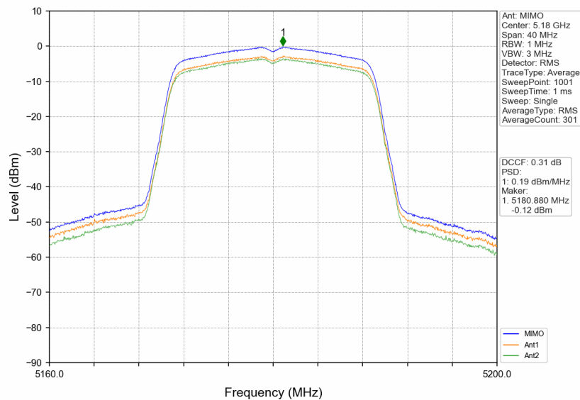
802.11ac(VHT20)_LCH_5180MHz_MIMO_NTNV
