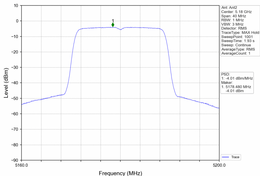
802.11ac(VHT20)_LCH_5180MHz_MIMO_NTNV
