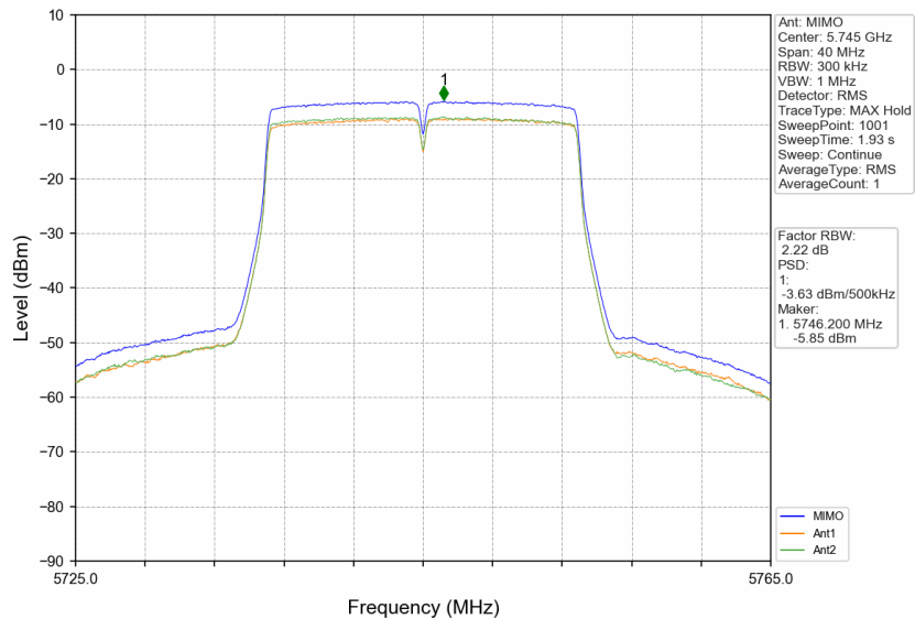
802.11ac(VHT20)_LCH_5745MHz_MIMO_NTNV
