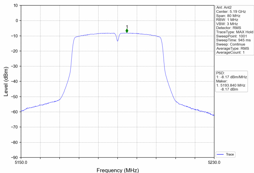
802.11n(HT40)_LCH_5190MHz_MIMO_NTNV
