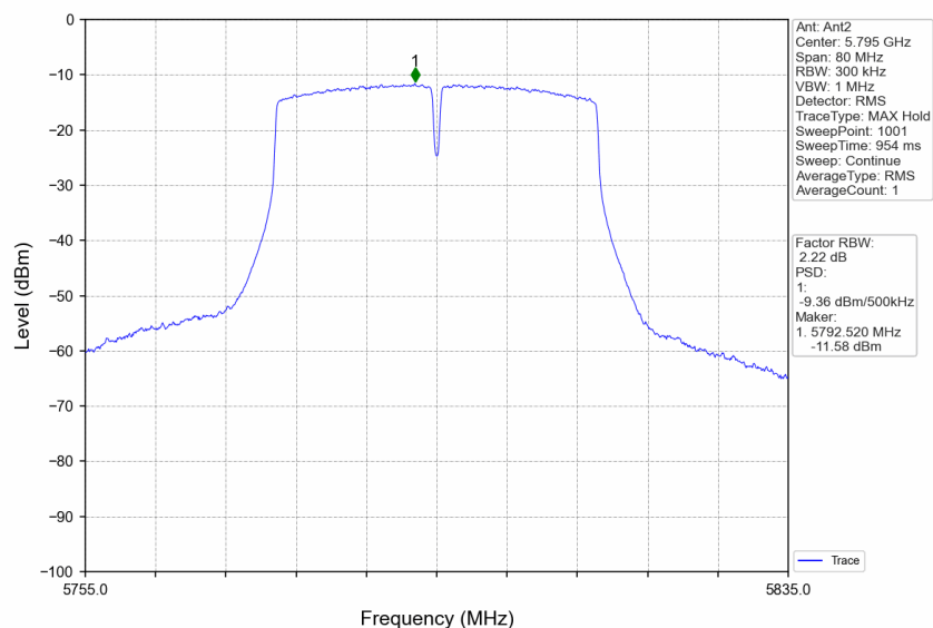
802.11ac(VHT40)_HCH_5795MHz_MIMO_NTNV
