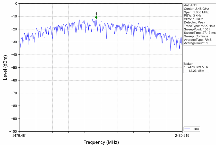
1M_HCH_2480MHz_DataRate= Ant1_NTNV
