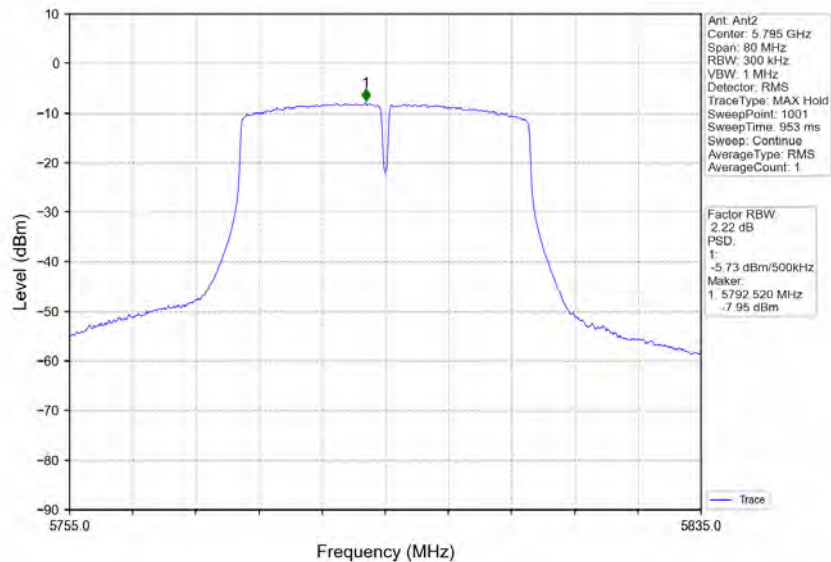
802.11ac(VHT40)_HCH_5795MHz_MIMO_NTNV
