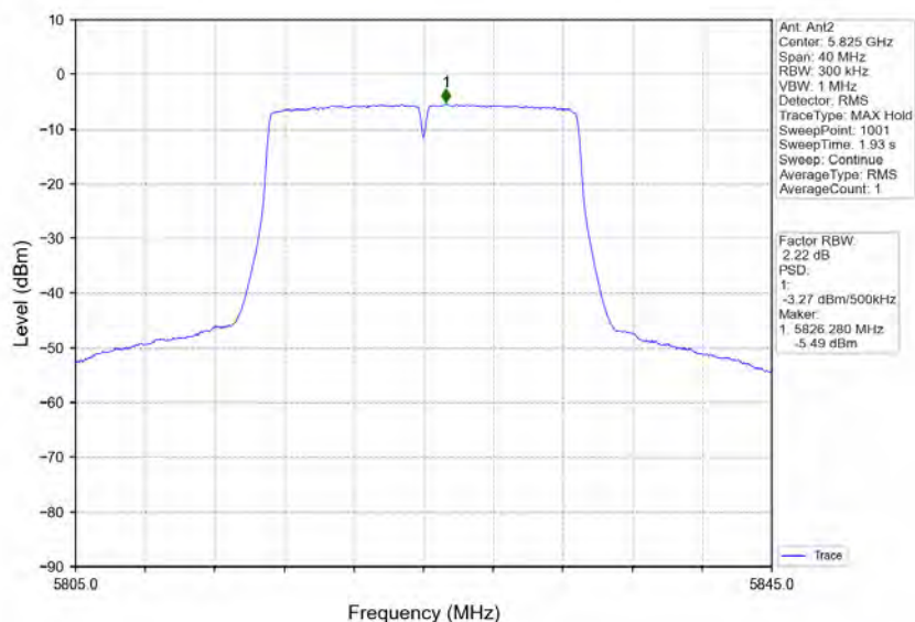
802.11ac(VHT20)_HCH_5825MHz_MIMO_NTNV
