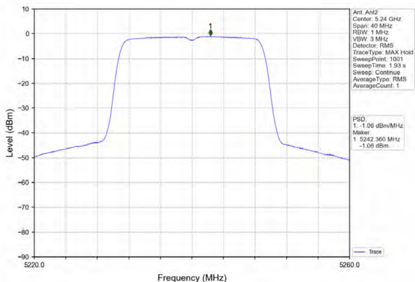
802.11ac(VHT20)_HCH_5240MHz_MIMO_NTNV
