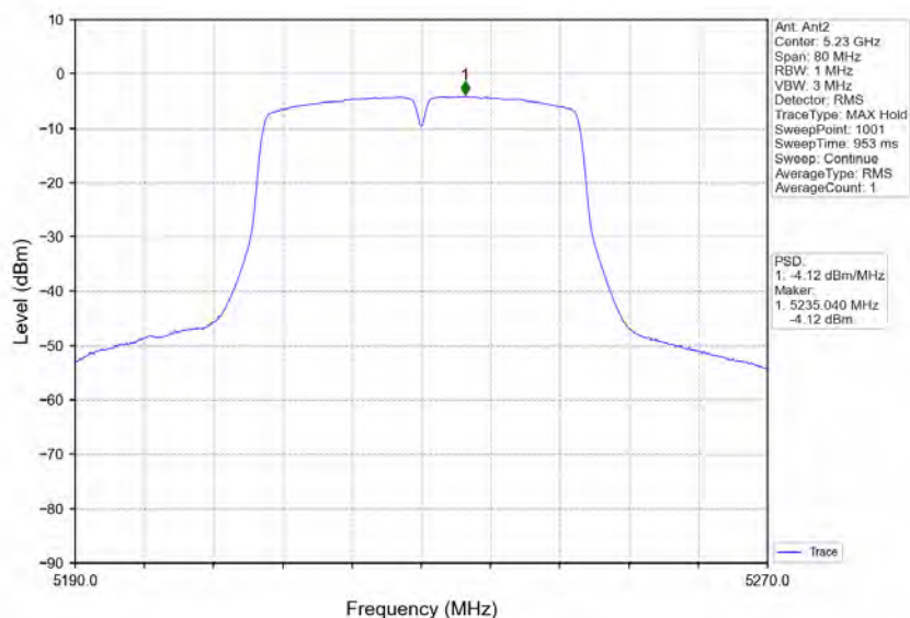
802.11ac(VHT40)_HCH_5230MHz_MIMO_NTNV
