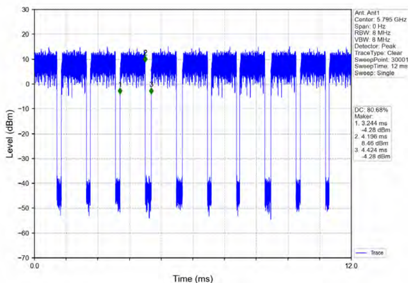
802.11ac(VHT40)_HCH_5795MHz_Ant1_NTN
