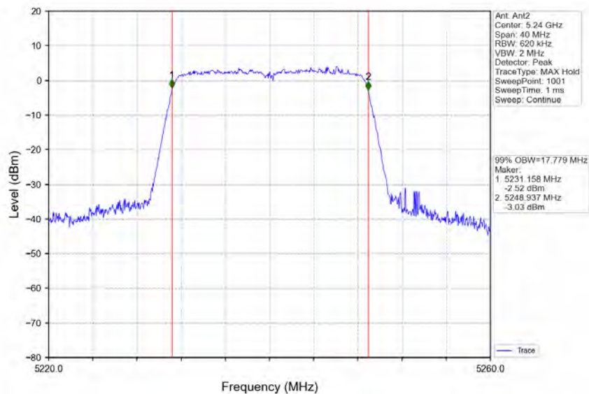
802.11n(HT20)_HCH_5240MHz_Ant2_NTNV
