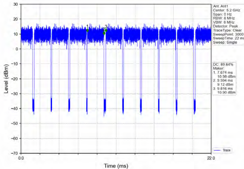
802.11n(HT20)_MCH_5200MHz_Ant1_NTN
