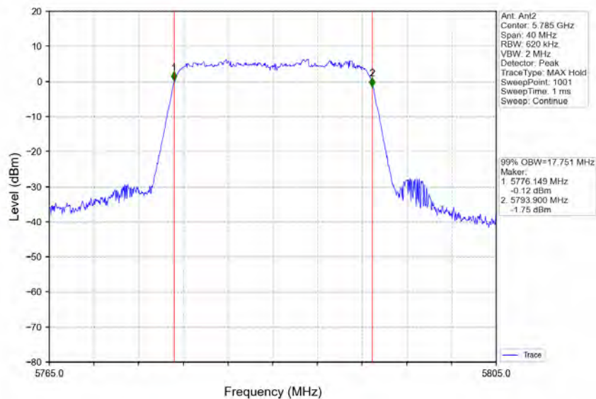
802.11ac(VHT20)_MCH_5785MHz_Ant2_NTNV
