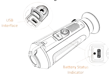
Figure 2-1 USB Interface
