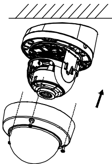
Figure 2-25 Install the Bubble
