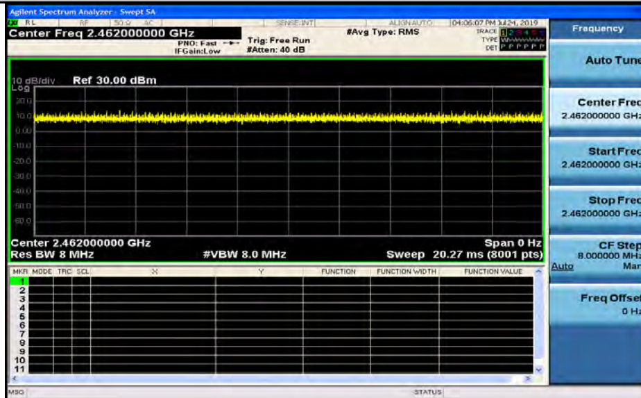
Duty Cycle_11G_2462_Ant2
