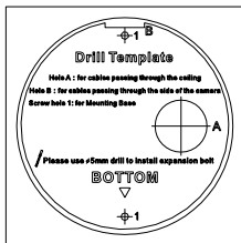
Figure 2-7 Drill Template B
