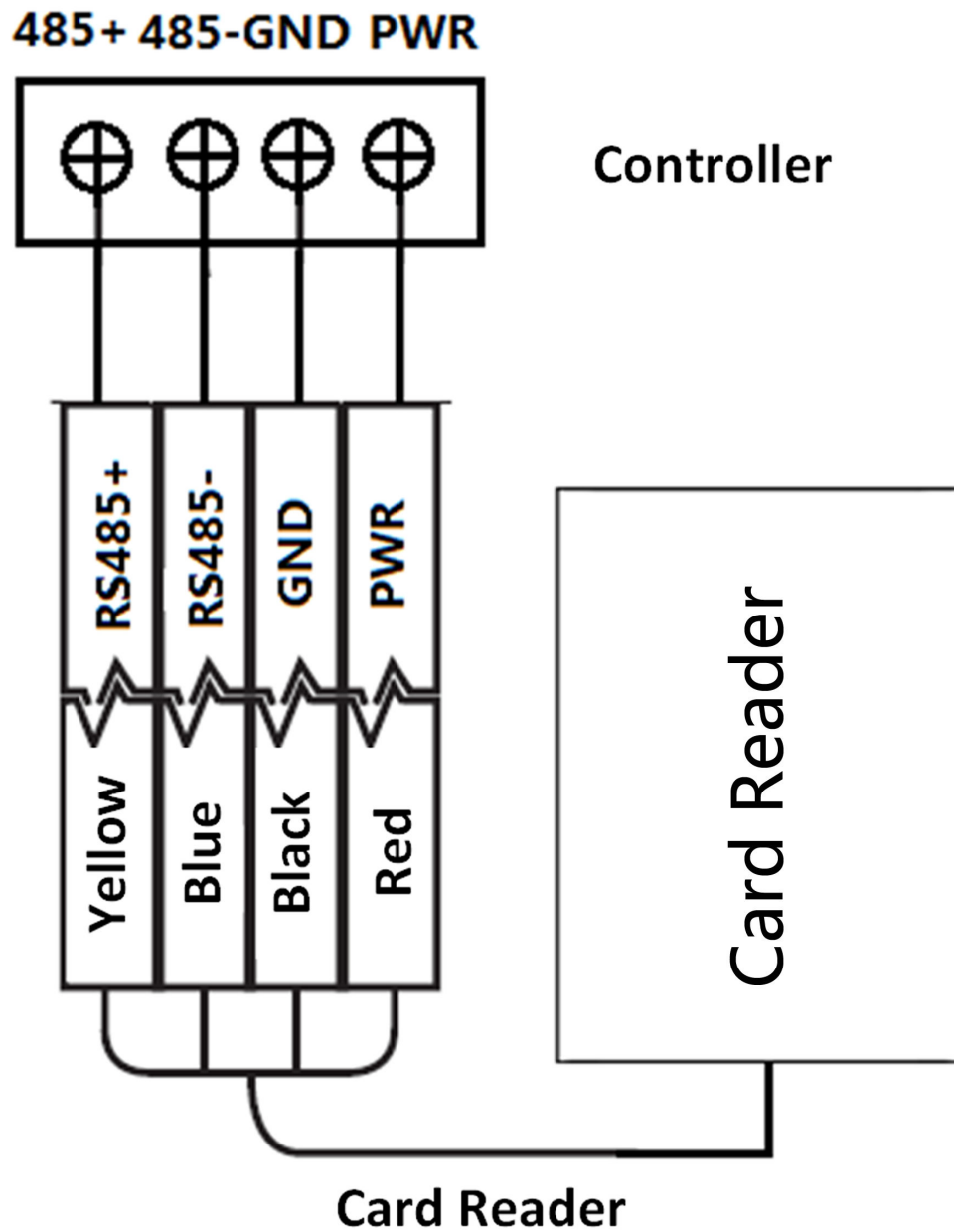
Figure 3-1 Wiring for RS-485 Communication Mode
