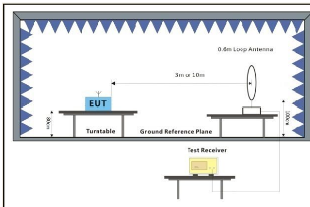
Below 30MHz
