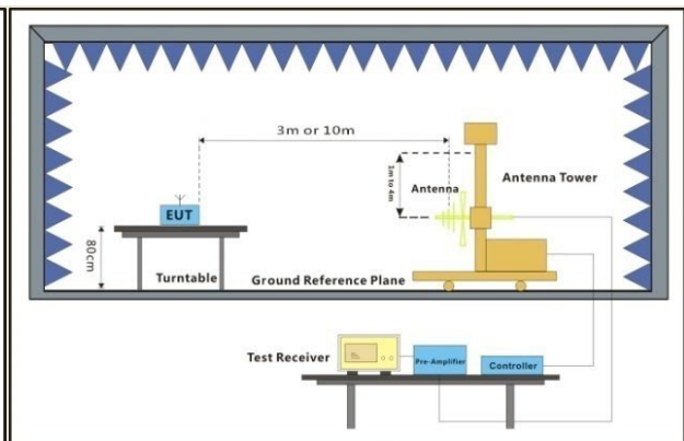
30MHz-1GHz
