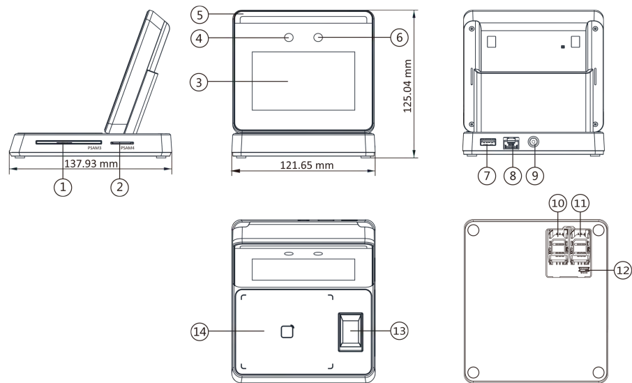
Figure 2-1 Appearance
