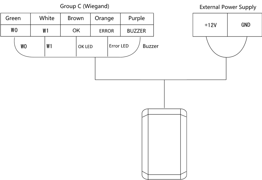
Figure 4-4 Wiring of Wiegand Card Reader
