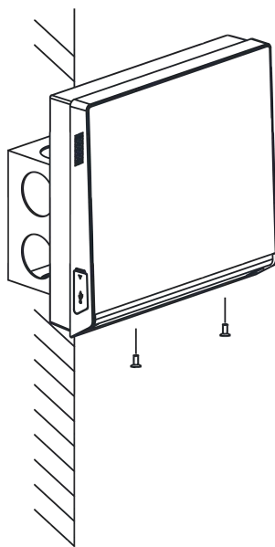
Figure 3-8 Tighten Screws
