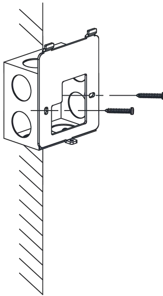
Figure 3-2 Install Mounting Plate
