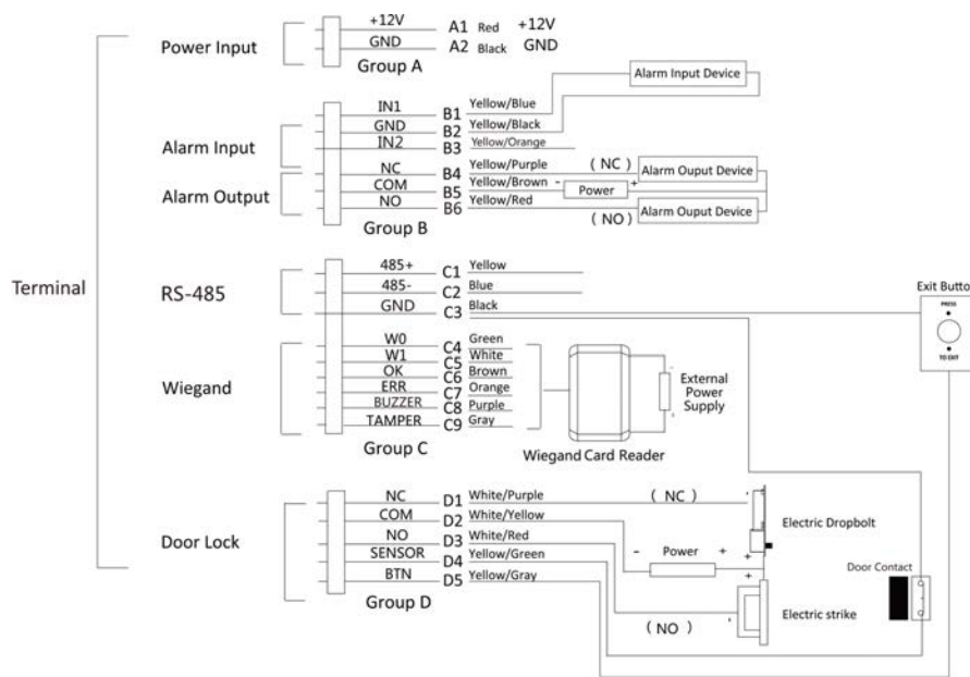
Figure 4-2 Wiring Overview
