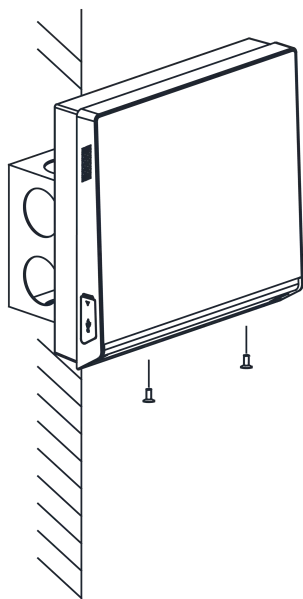
Figure 3-8 Tighten Screws
