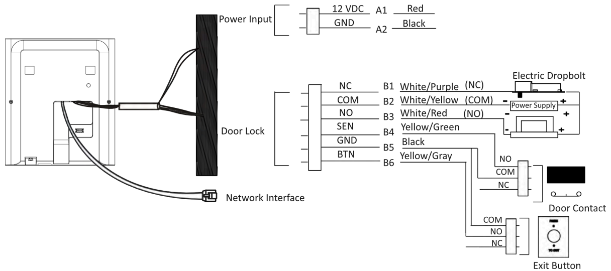
Figure 4-1 Device Wiring
