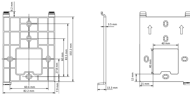
Figure 3-5 Mounting Template
