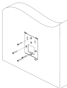
Figure 3-2 Install Mounting Plate
