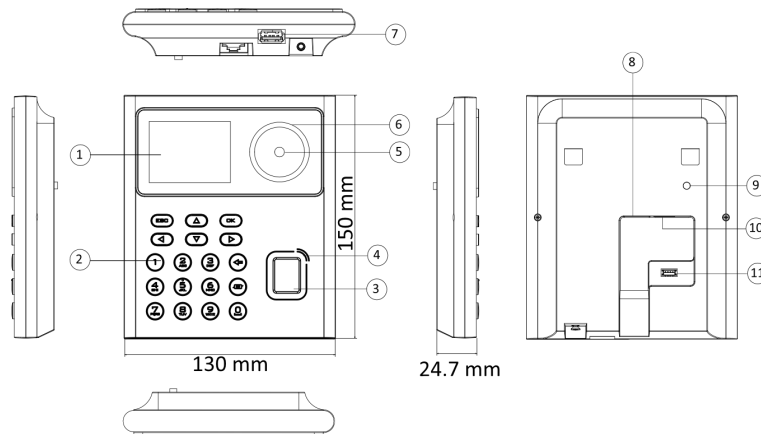
Figure 2-1 Appearance (With Fingerprint)
