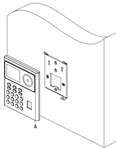
Figure 3-4 Secure Device
