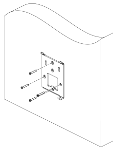
Figure 3-6 Install Mounting Plate
