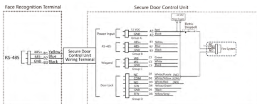
Figure 4-6 Wiring Secure Door Control Unit
