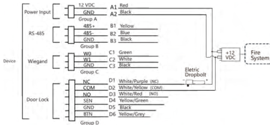
Figure 4-3 Wire Device
