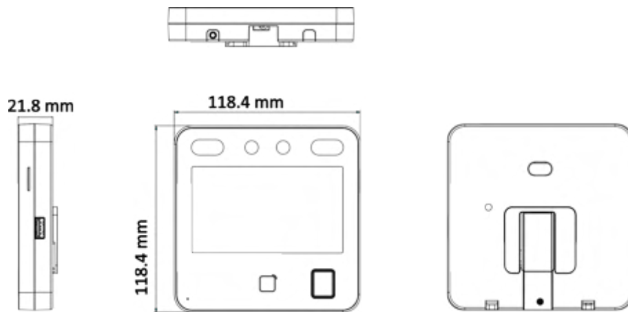
Figure D-1 Dimension (With Fingerprint)
