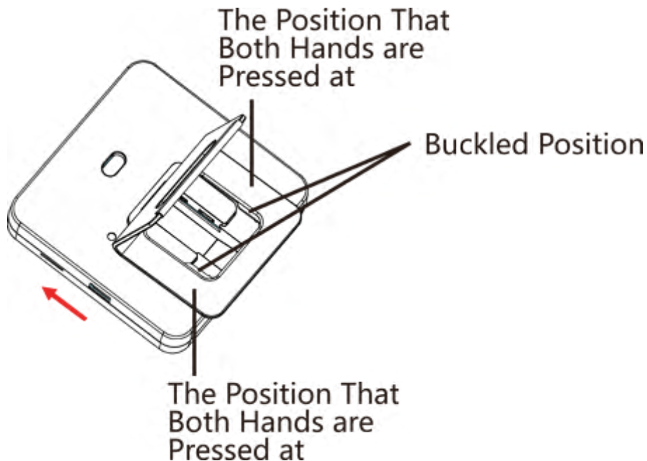
Figure 3-5 Fasten Bracket
