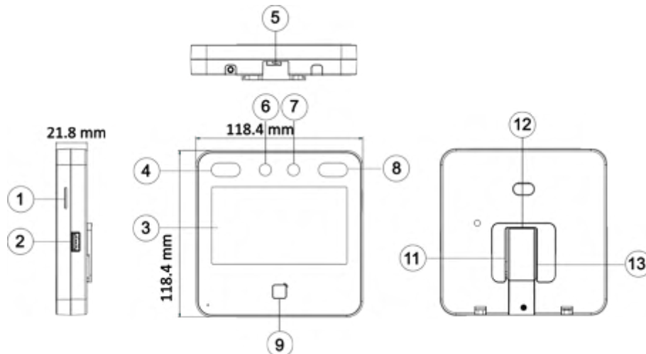
Figure 2-2 Appearance (Without Fingerprint)
