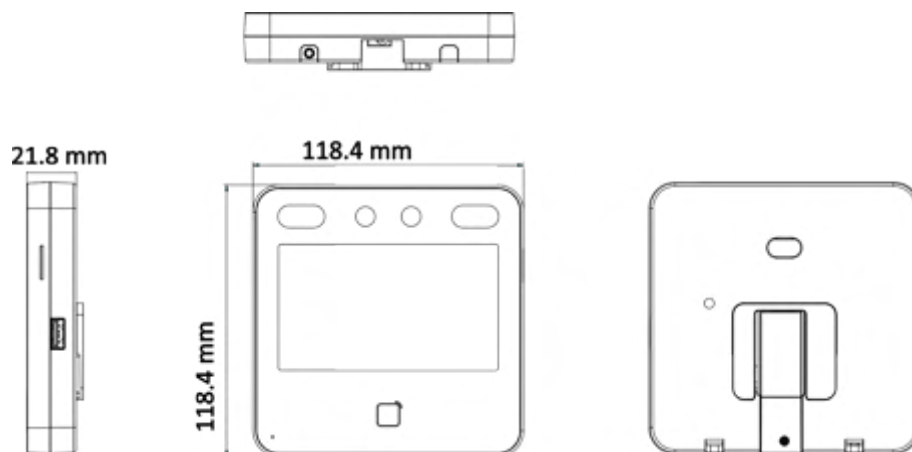
Figure D-2 Dimension (Without Fingerprint)
