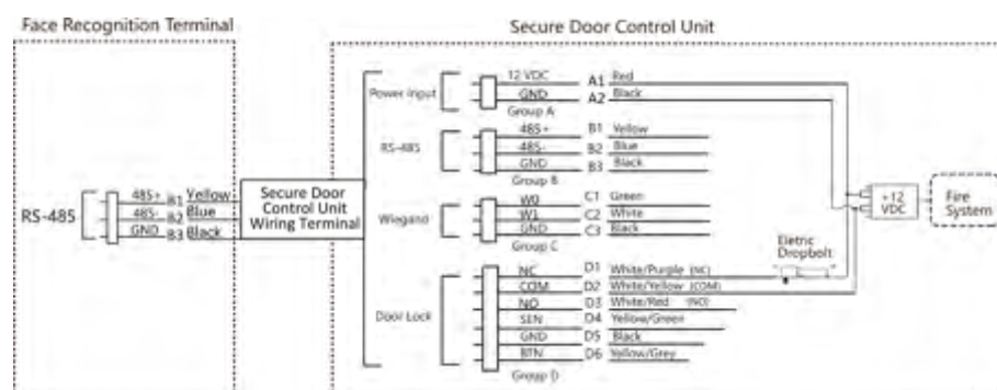
Figure 4-4 Wire Secure Door Control Unit
