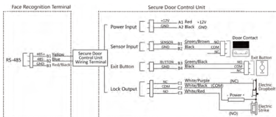
Figure 4-2 Secure Door Control Unit Wiring
