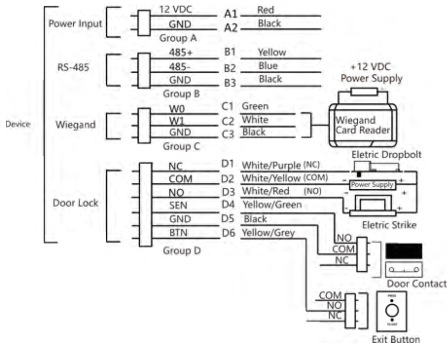
Figure 4-1 Device Wiring
