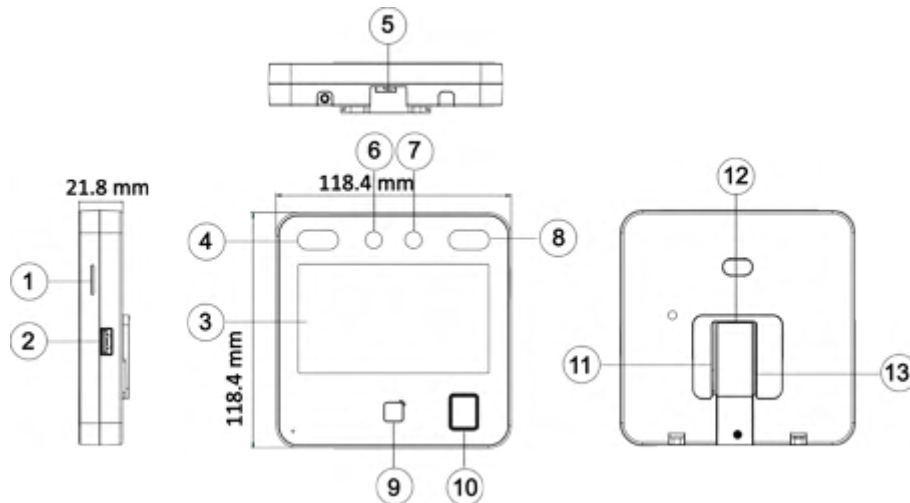
Figure 2-1 Appearance (With Fingerprint)
