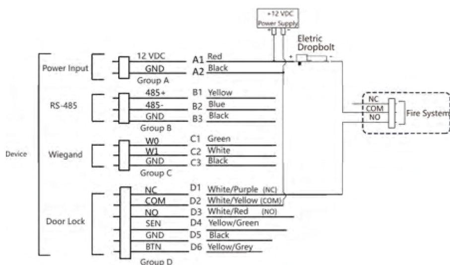
Figure 4-5 Wiring Device
