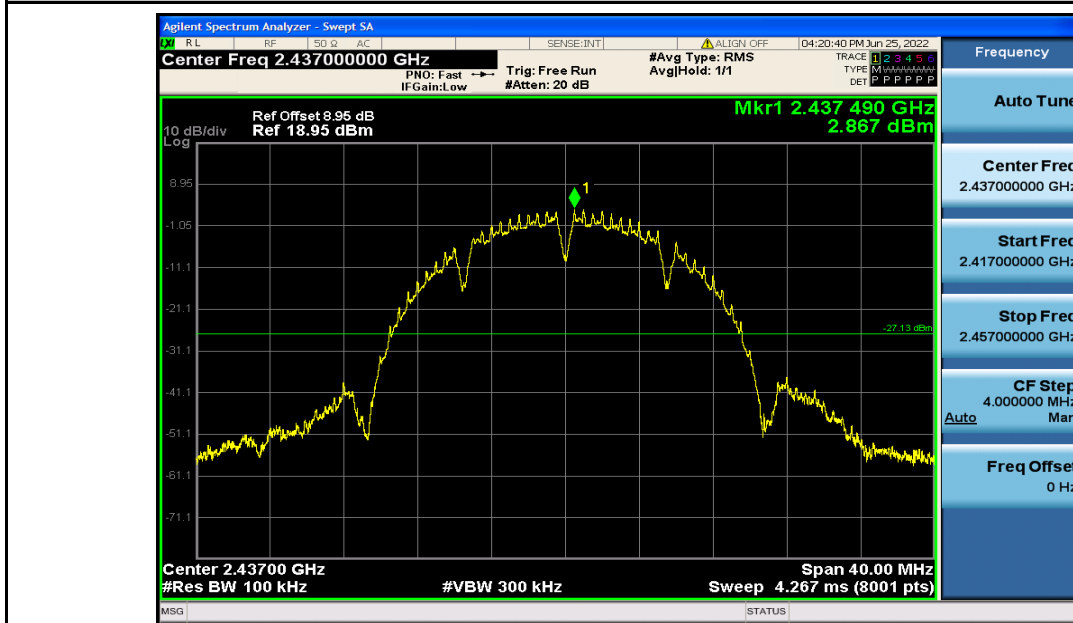
RF Conducted Spurious Emissions_11B_2437
