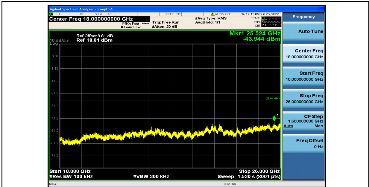
RF Conducted Spurious Emissions_11B_2437
