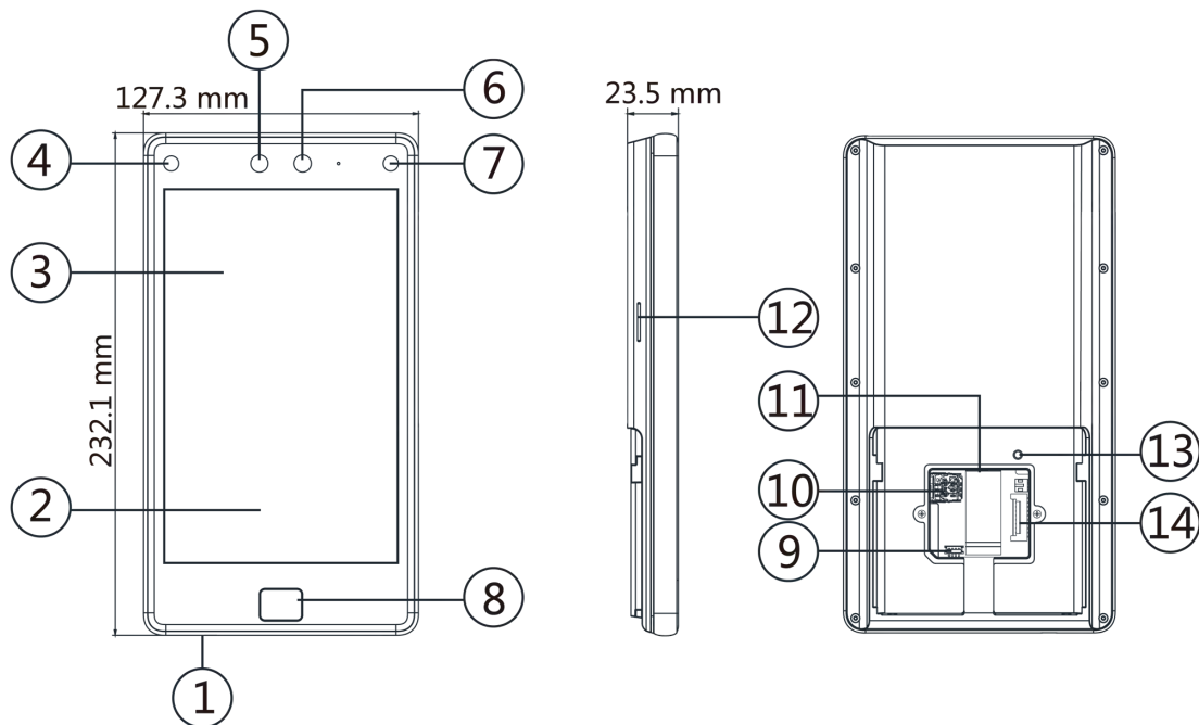
Figure 2-1 Face Recognition Terminal Diagram
