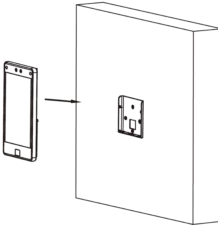
Figure 3-6 Hang Device
