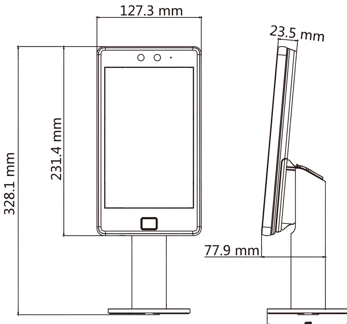
Figure D-2 Dimension with Bracket
