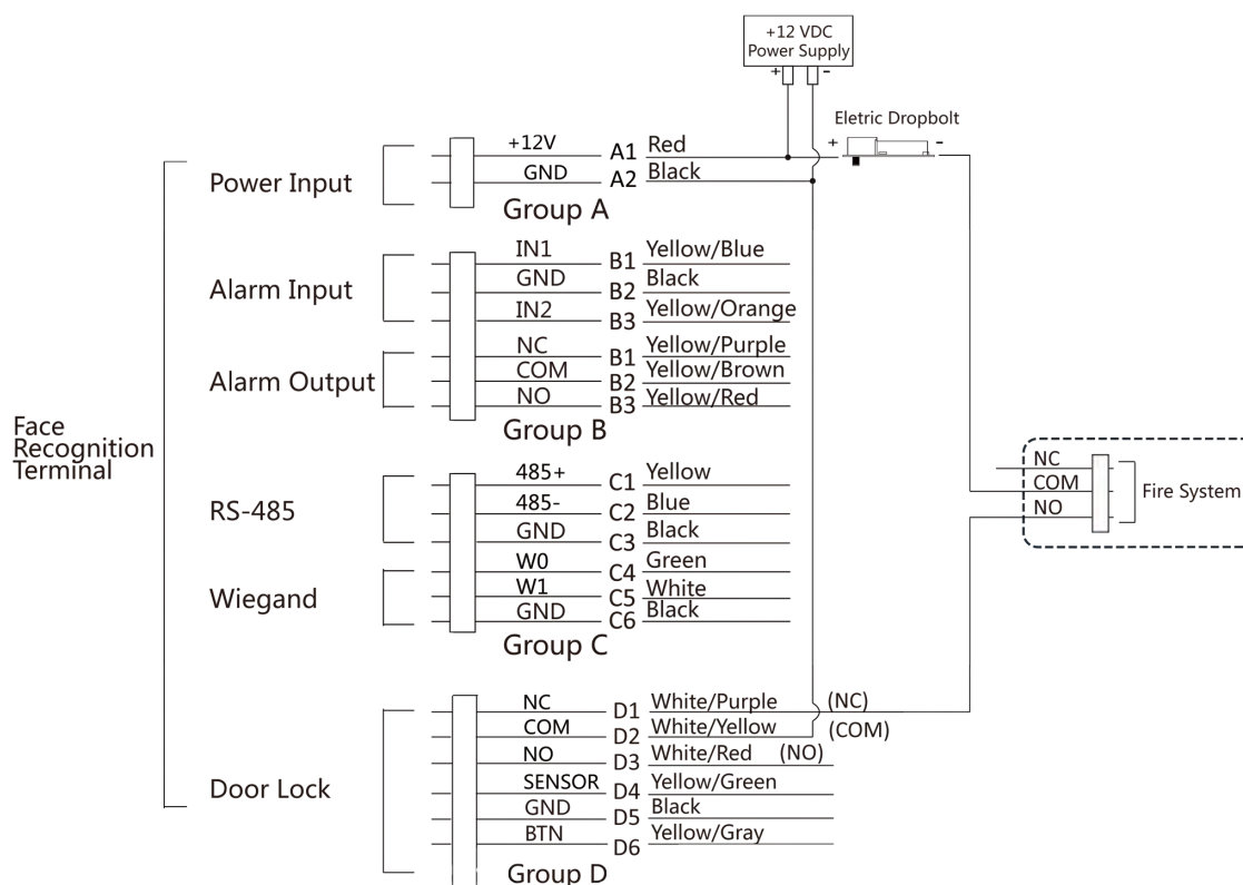
Figure 4-6 Wiring Device
