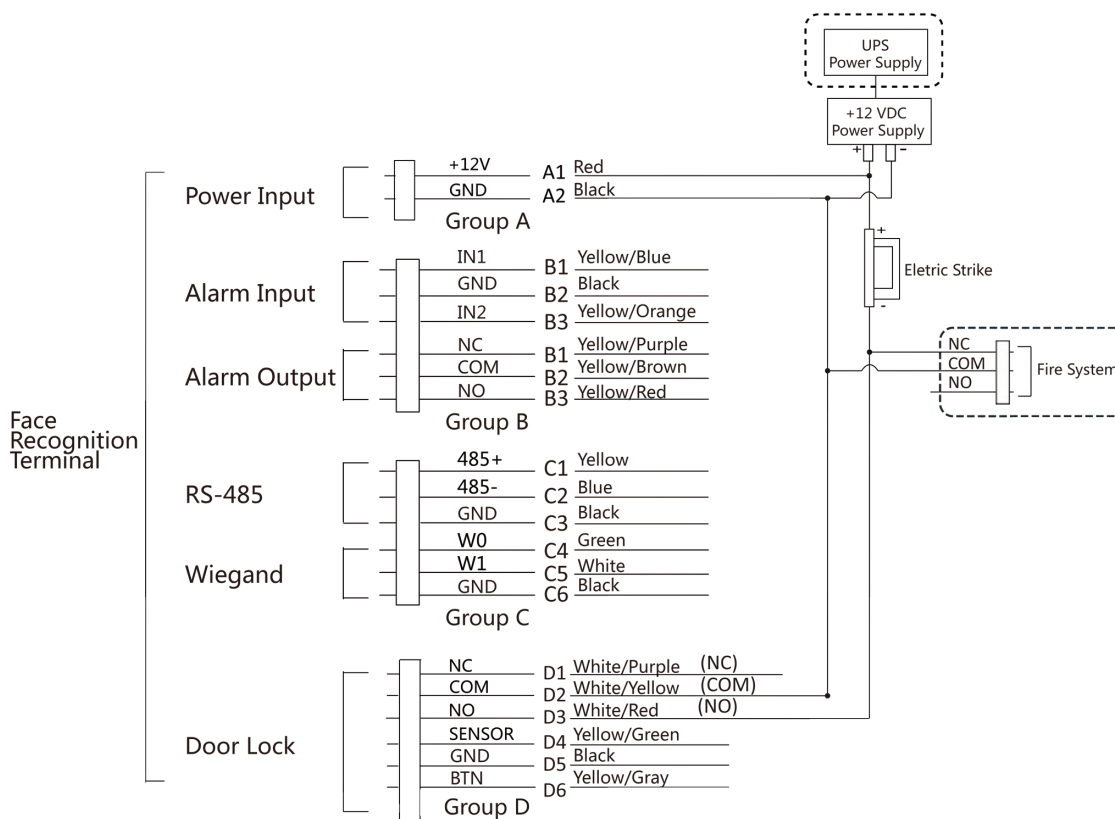
Figure 4-8 Device Wiring
