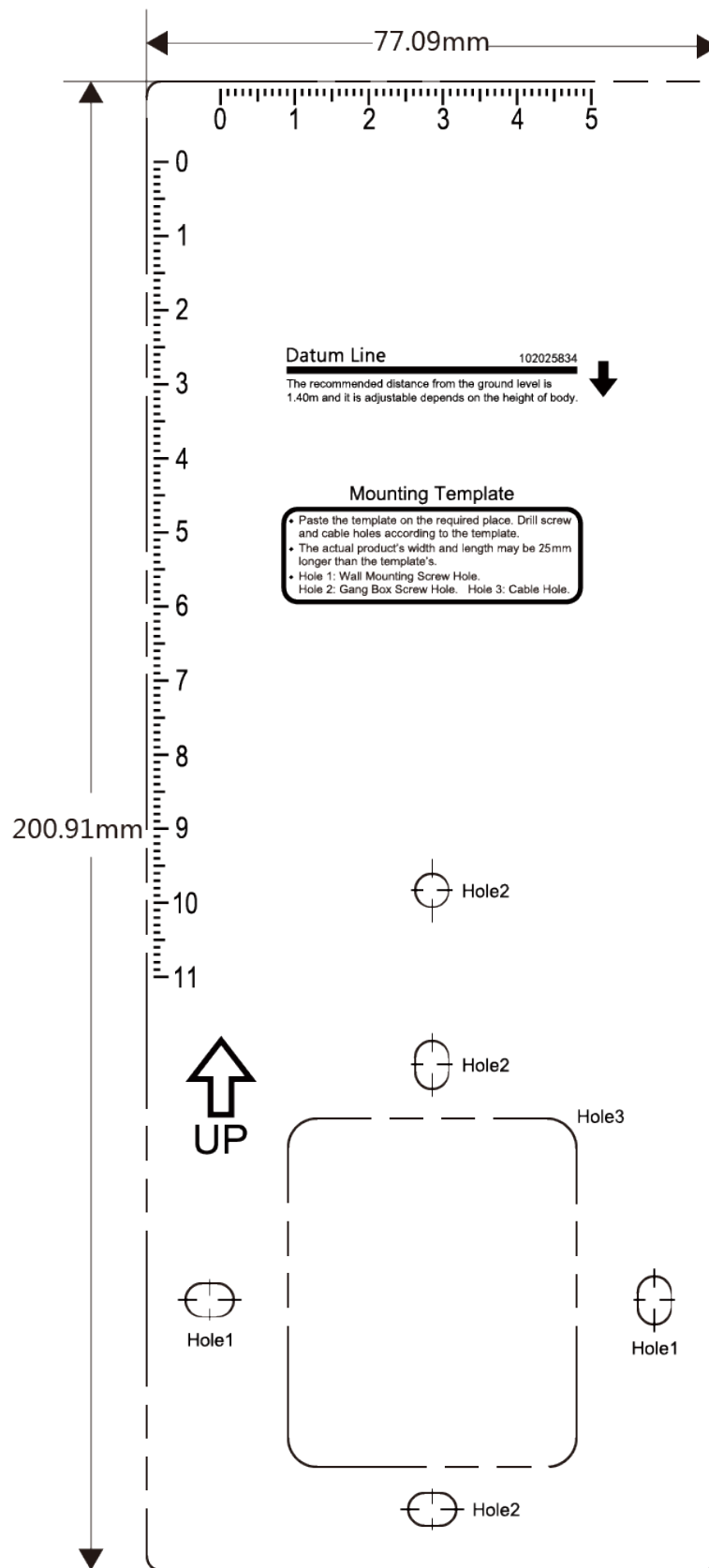
Figure 3-4 Mounting Template
