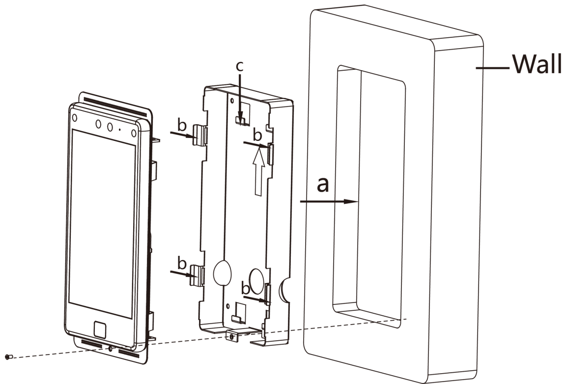
Figure 3-3 Secure the Combination and the Gang Box
