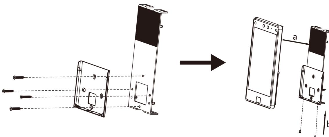
Figure 3-1 Secure the Device on the mounting plate
