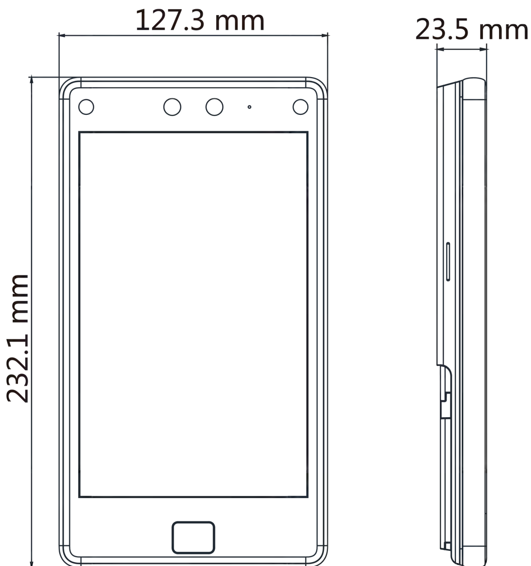
Figure D-1 Dimension
