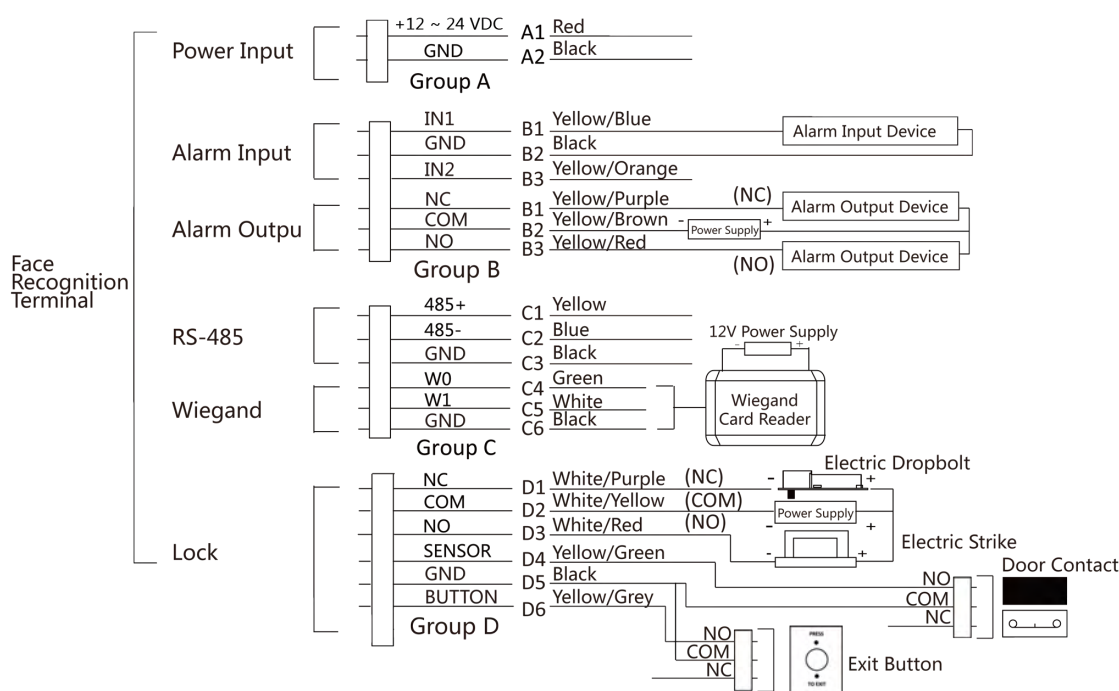
Figure 4-2 Device Wiring
