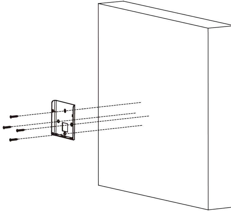
Figure 3-5 Install Mounting Plate
