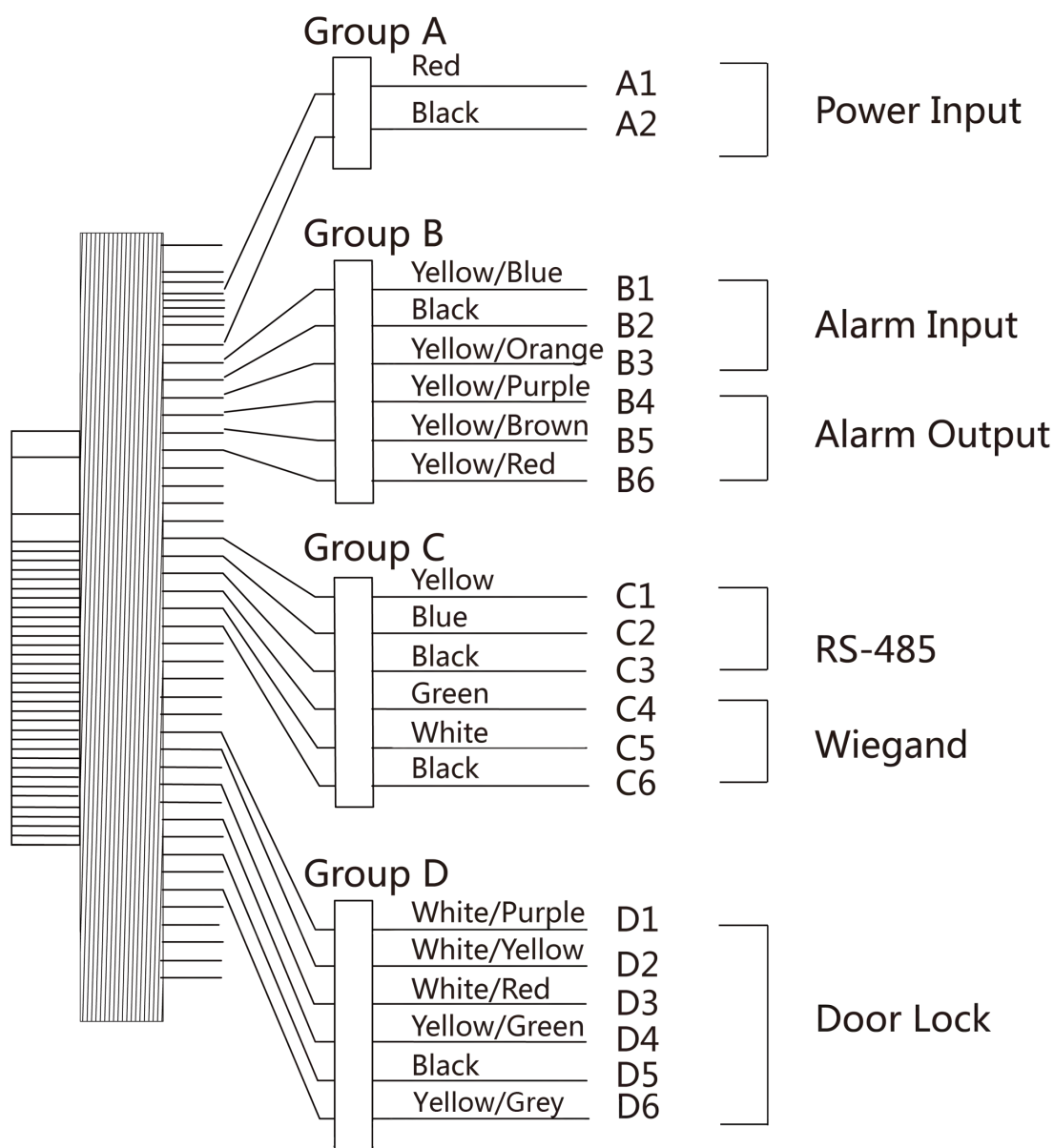
Figure 4-1 Terminal Diagram
