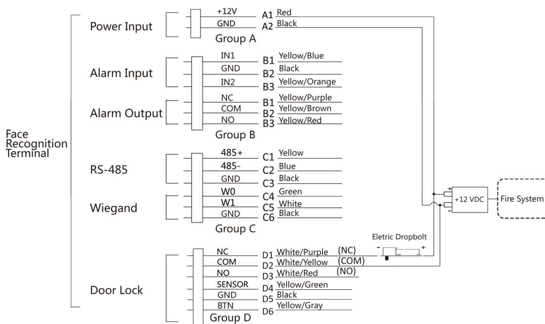
Figure 4-4 Wire Device
