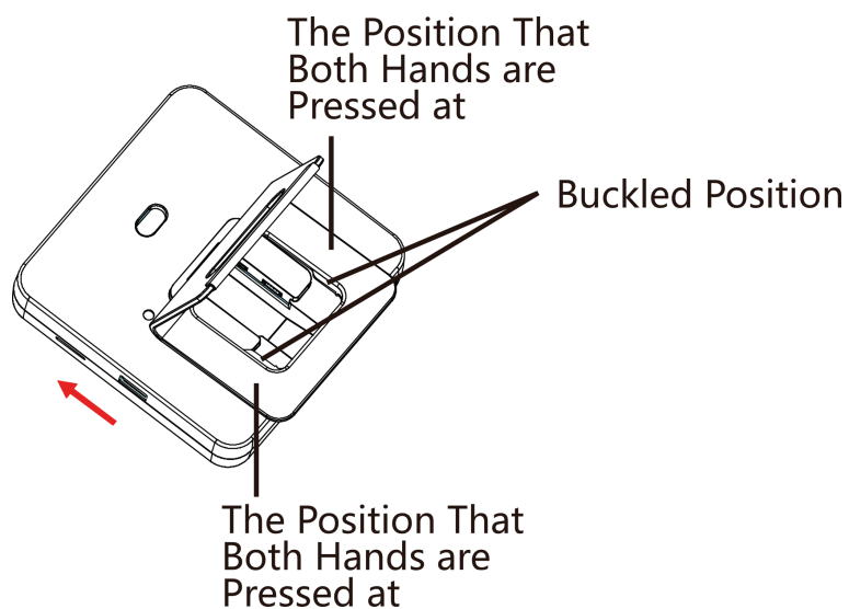
Figure 3-5 Fasten Bracket
