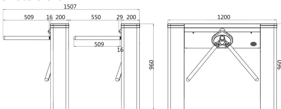
Figure 2-2 Dimension
