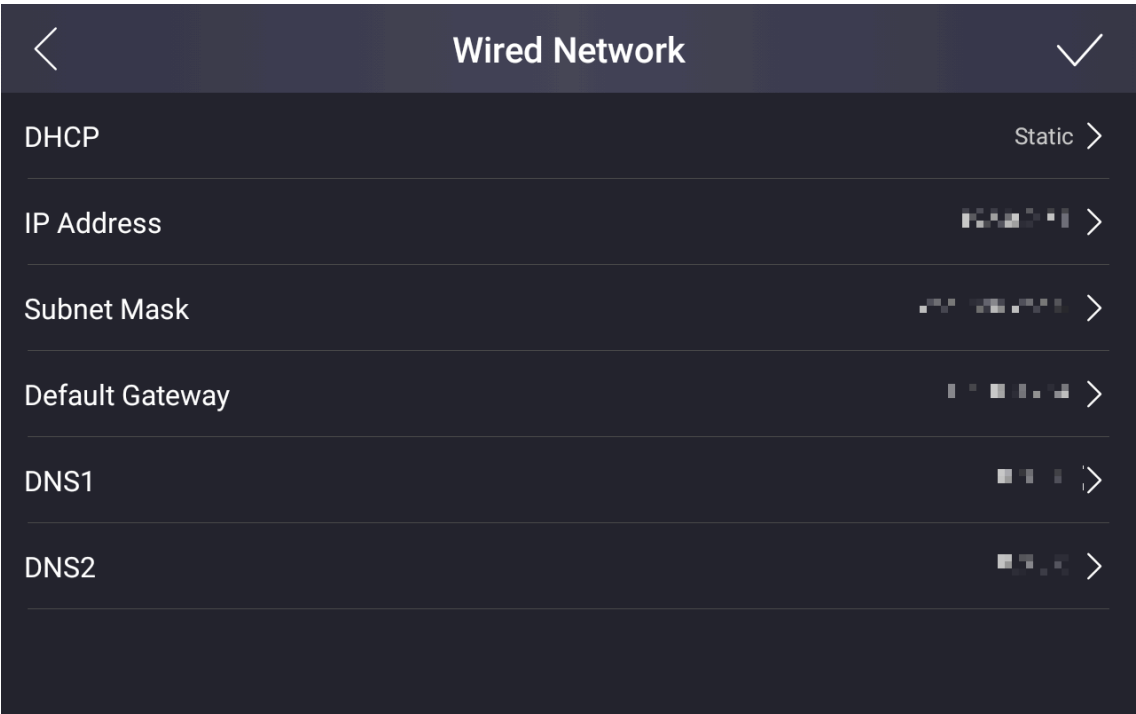
Figure 7-11 Wired Network
