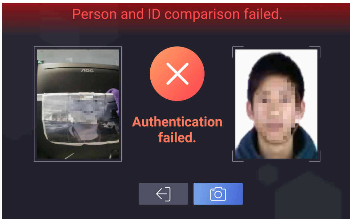
Figure 7-9 Failed Authentication
