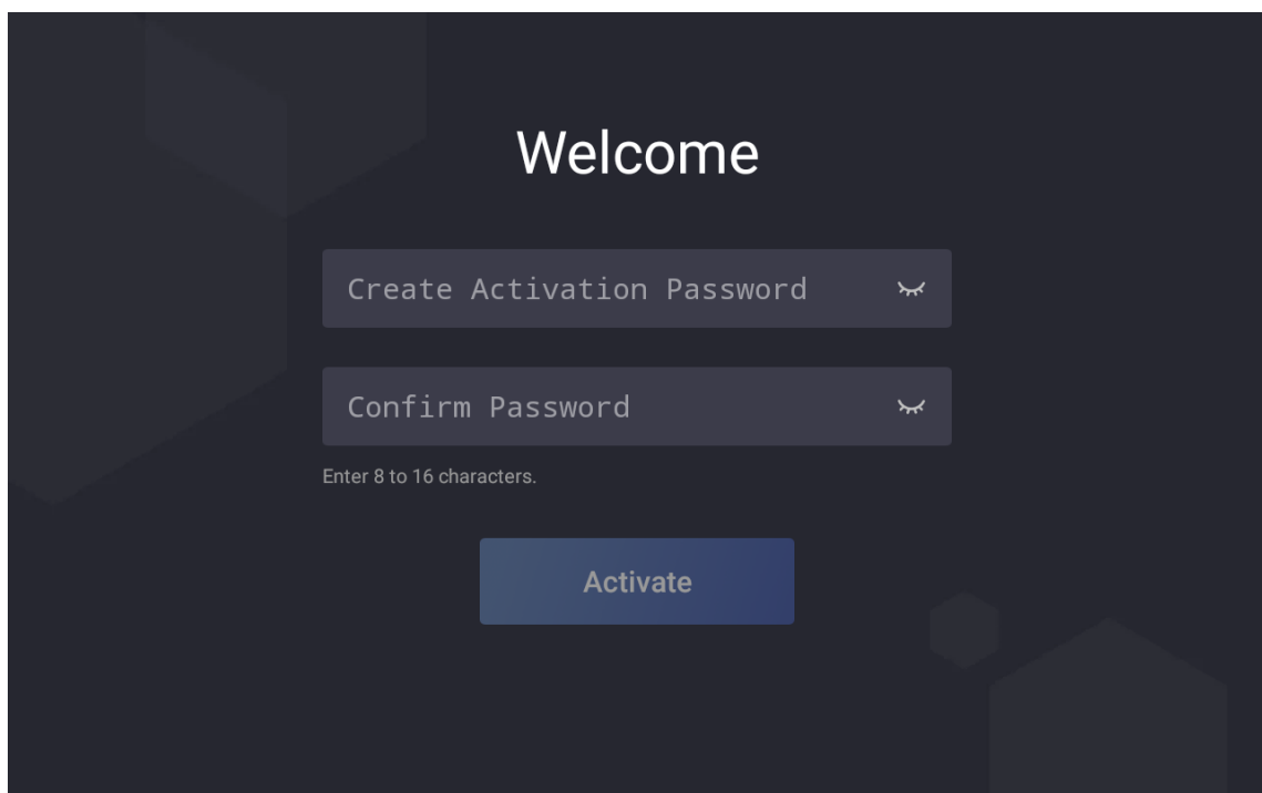
Figure 5-1 Activation Page
