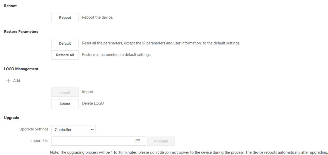
Figure 8-12 Logo Management
