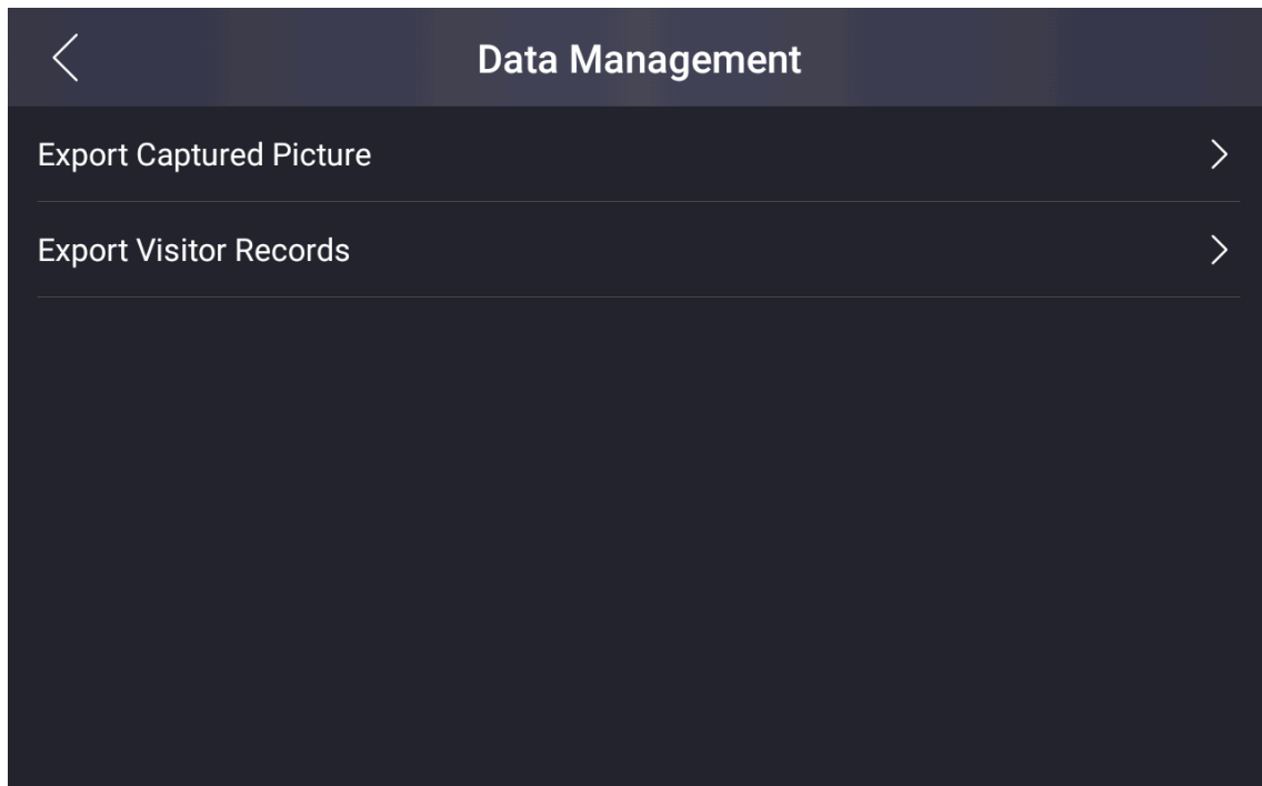
Figure 7-16 Data Management
