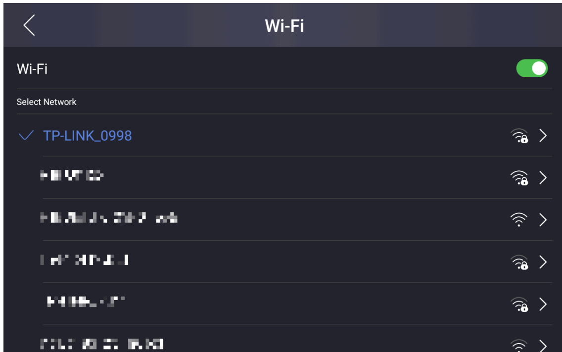
Figure 7-12 Wi-Fi
