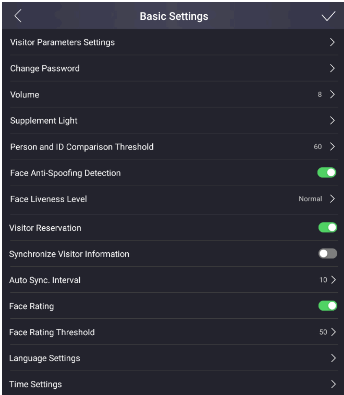
Figure 7-14 Basic Parameters
