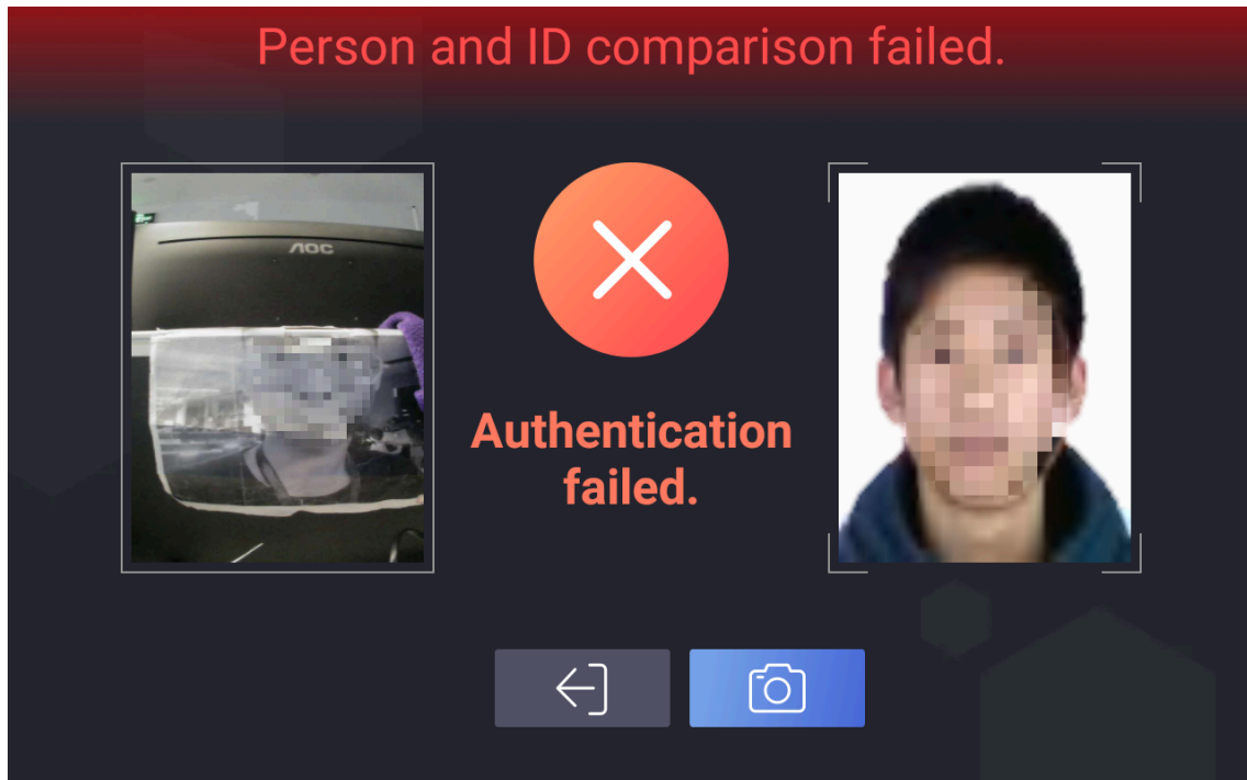
Figure 7-2 Failed Authentication
