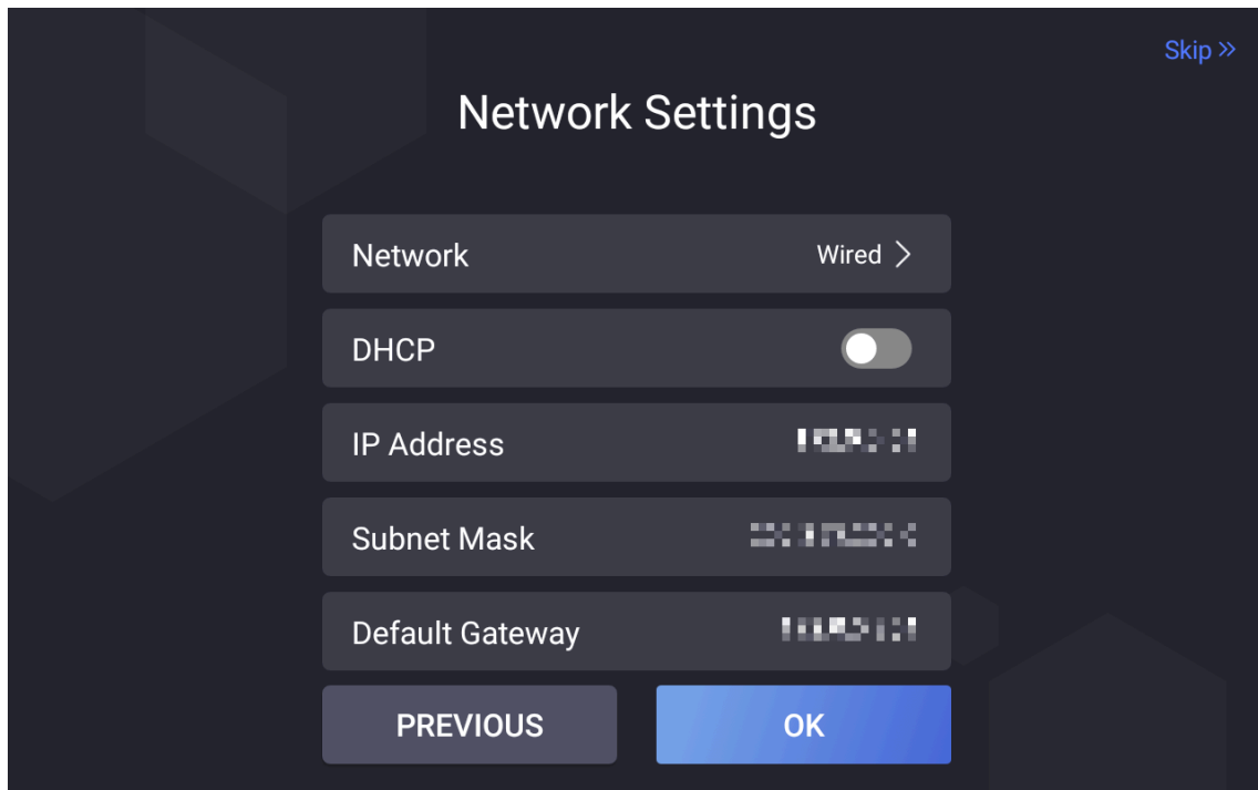
Figure 7-20 Set Network
